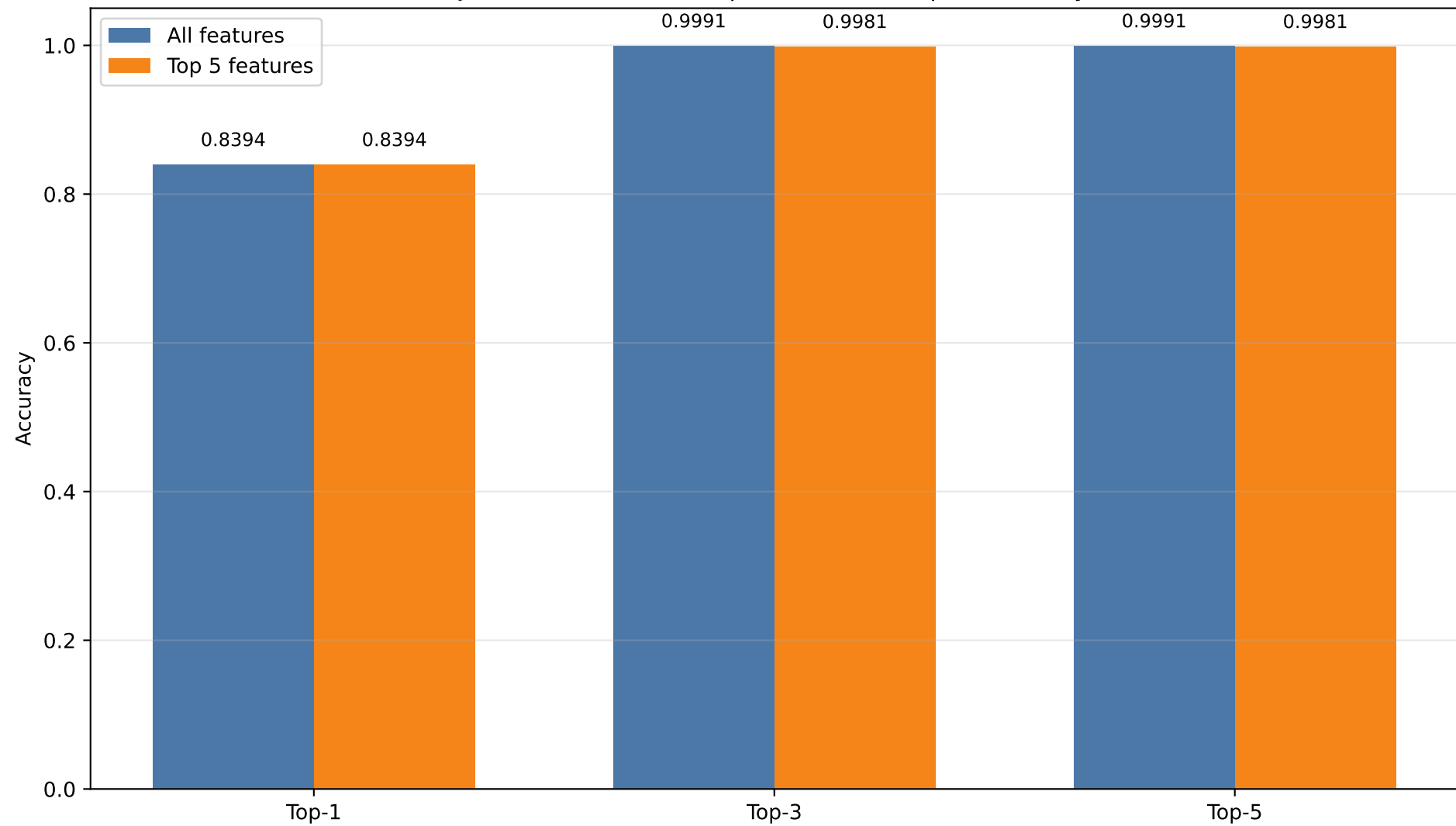
JA4 SNI features vs Top 5 features - Top-k accuracy
