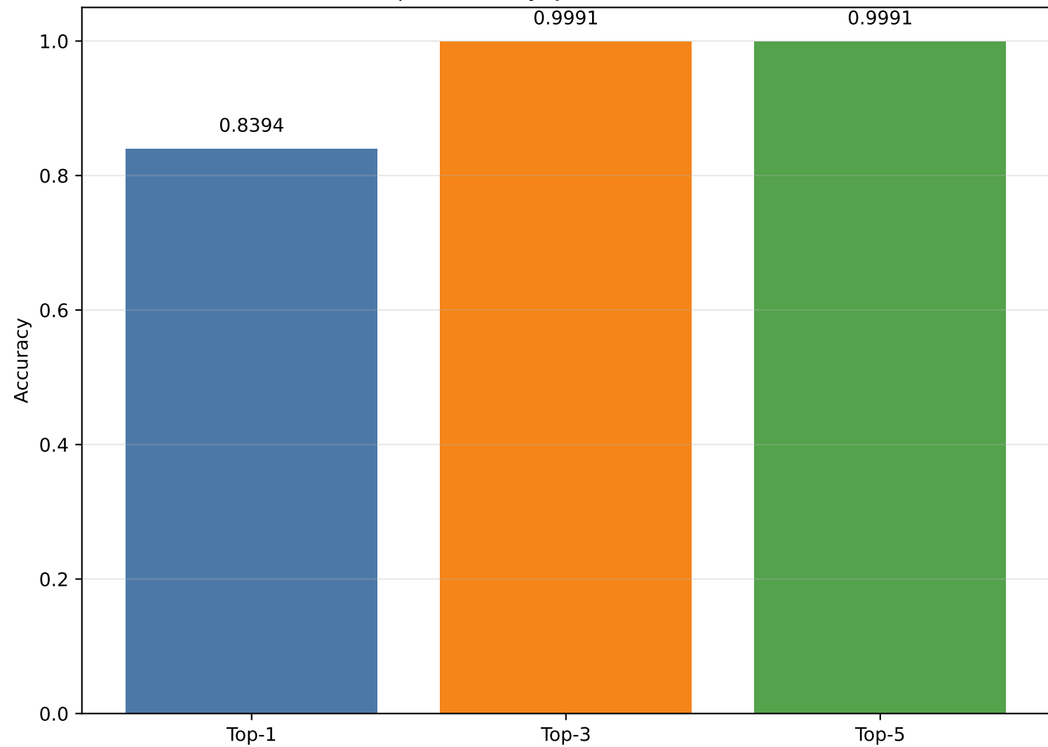
Top-k accuracy (JA4+SNI features)
