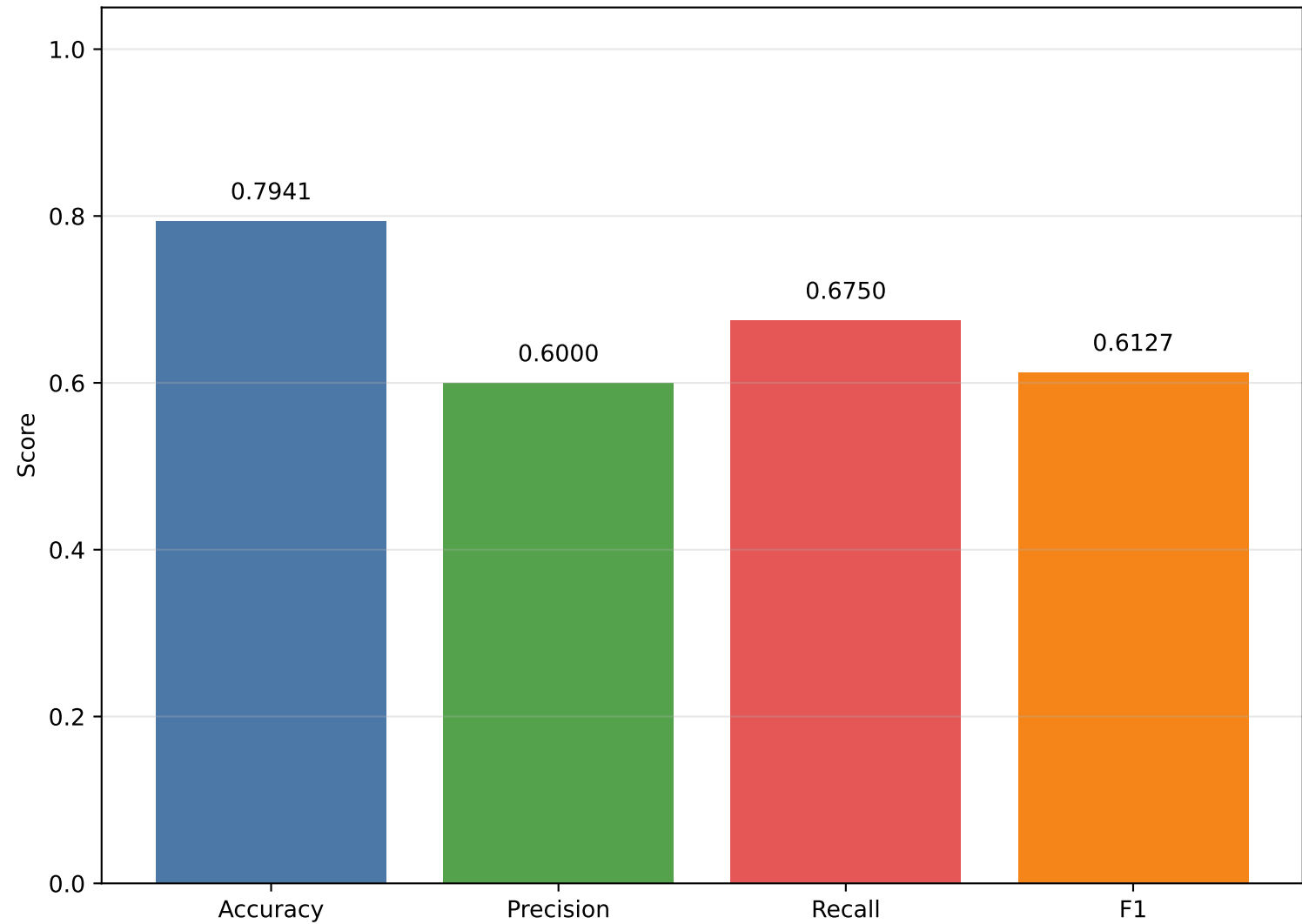
Test Metrics (JA4 + JA4S + JA4TS complete fingerprints)
