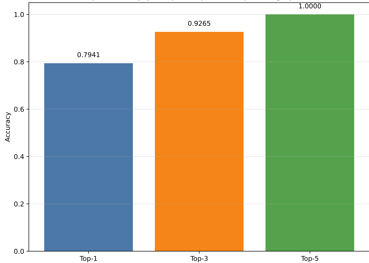
Top-k accuracy (JA4 + JA4S + JA4TS complete fingerprints)
