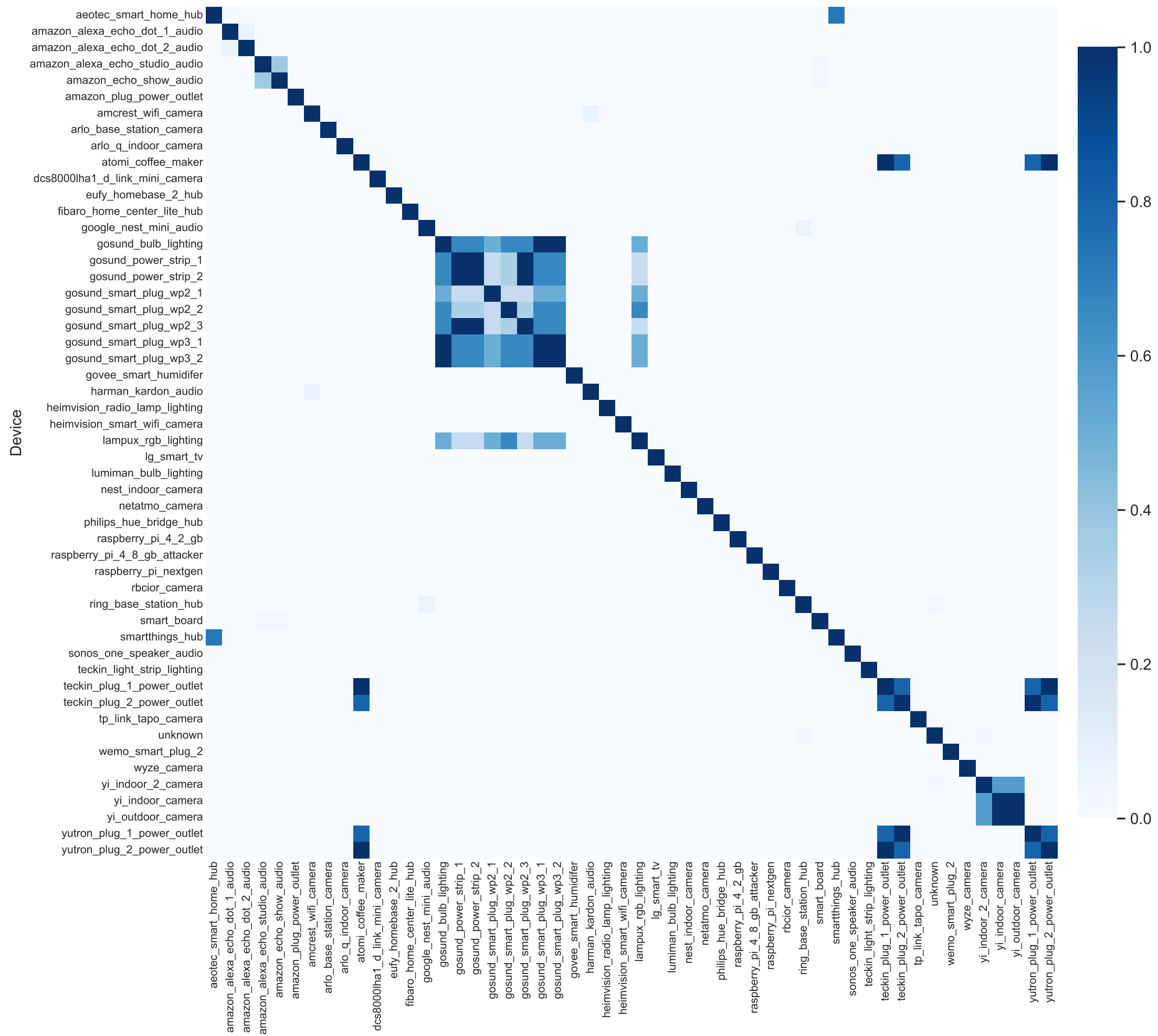
Similarity matrix JA4+JA4S+JA4T+JA4TS Fingerprints
