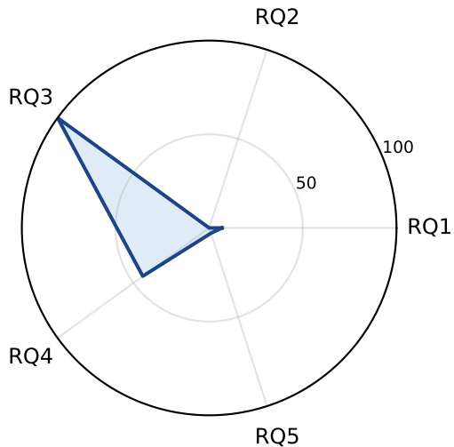
Ignite
