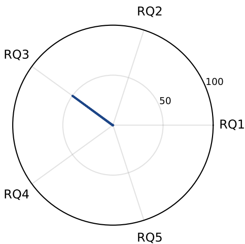
MSSQL/Microsoft Azure
