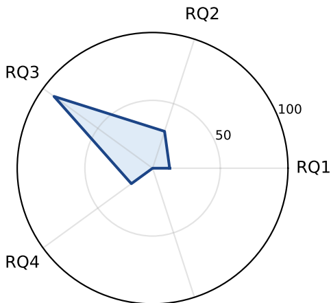
MSSQL/Microsoft Azure
