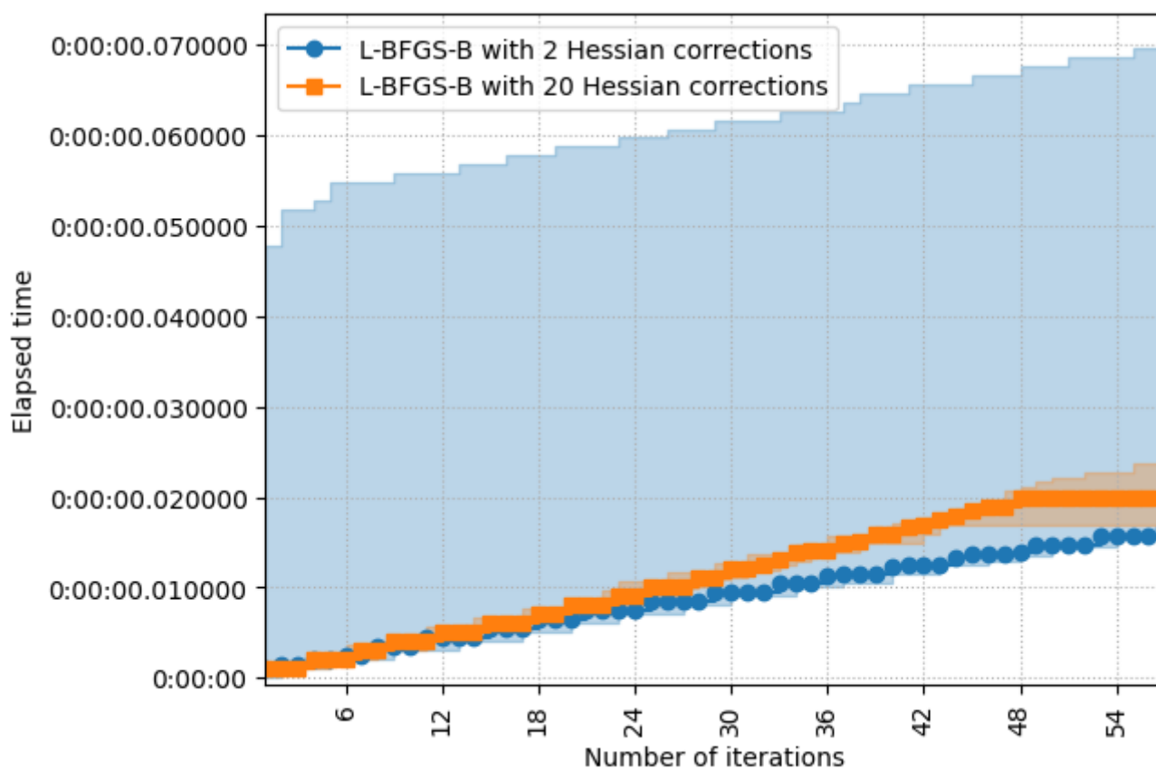
The execution time of group L-BFGS-B configurations for problem configuration Rosenbrock 5D.
