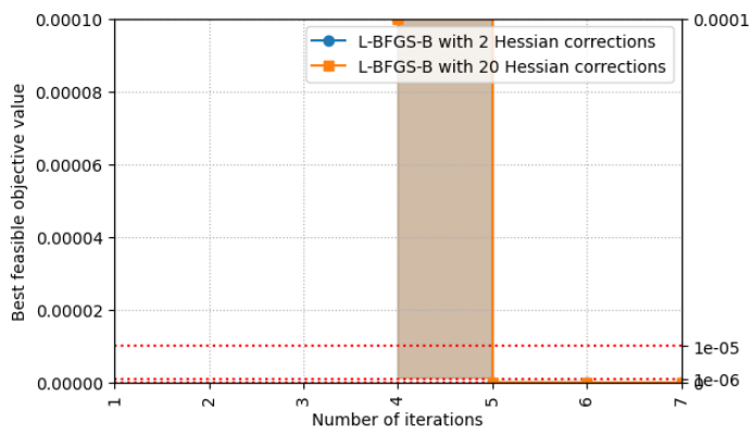
The best feasible objective value of group L-BFGS-B configurations for problem configuration Rastrigin.
