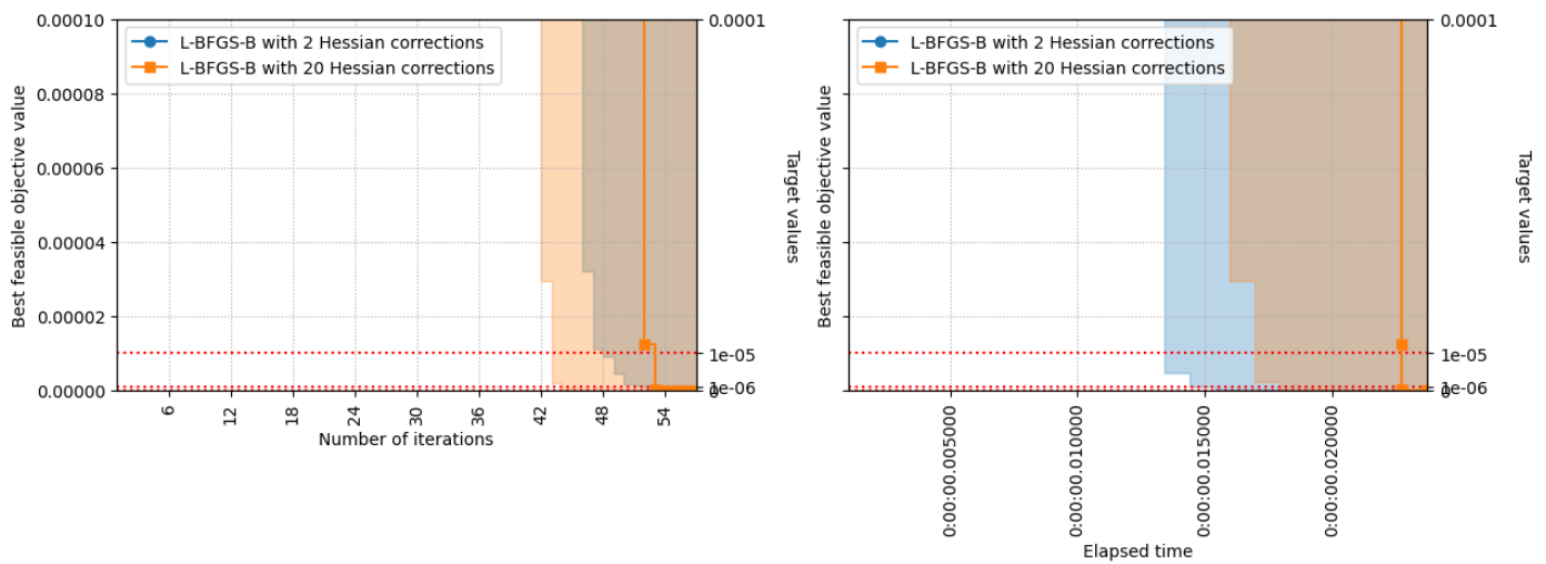
The best feasible objective value of group L-BFGS-B configurations for problem configuration Rosenbrock 5D.
