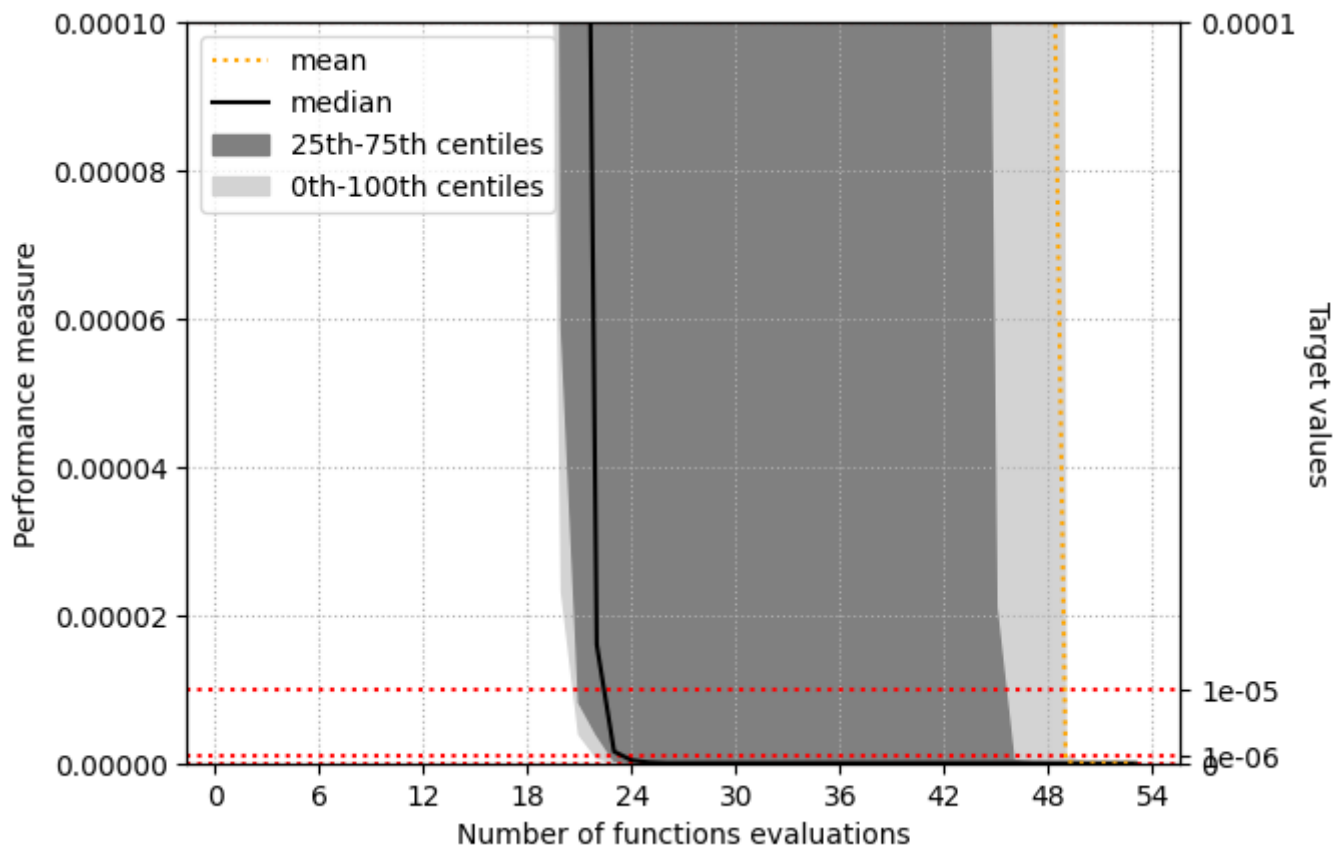
The performance measure of algorithm configuration 'L-BFGS-B with 2 Hessian corrections' for problem 'Rosenbrock'.
