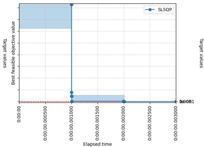
The best feasible objective value of group SLSQP for problem configuration Rastrigin.
