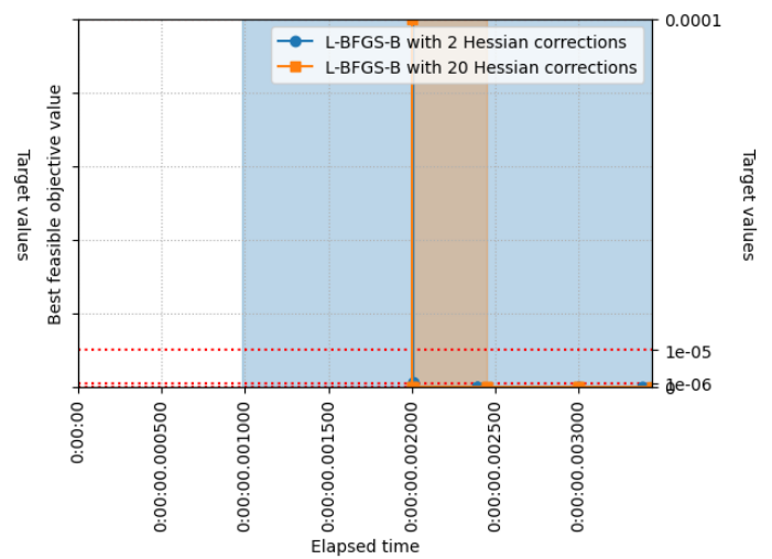
The best feasible objective value of group L-BFGS-B configurations for problem configuration Rastrigin.
