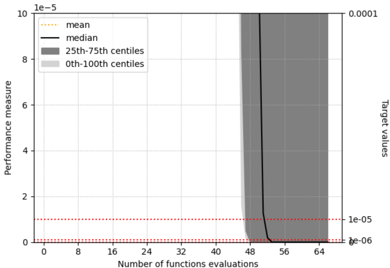
The performance measure of algorithm configuration 'SLSQP' for problem 'Rosenbrock 5D'.
