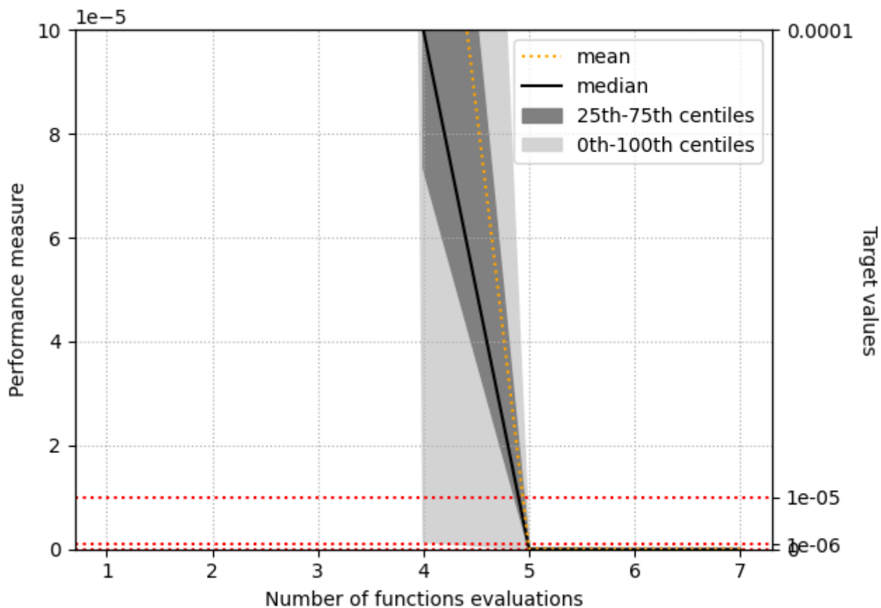
The performance measure of algorithm configuration 'L-BFGS-B with 20 Hessian corrections' for problem 'Rastrigin'.
