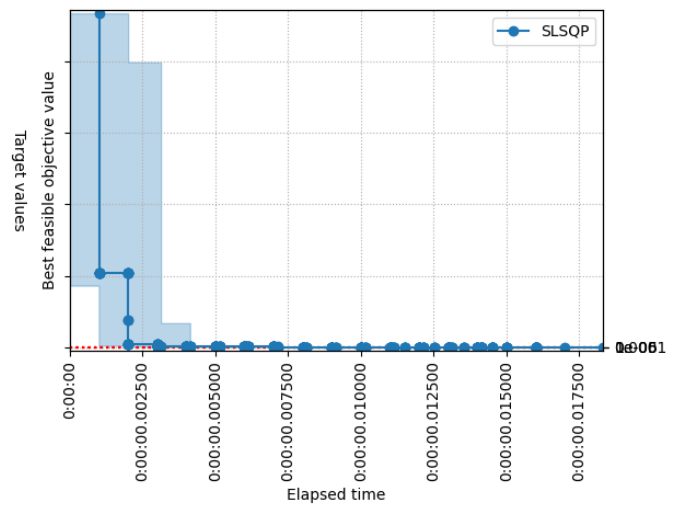
The best feasible objective value of group SLSQP for problem configuration Rosenbrock 5D.
