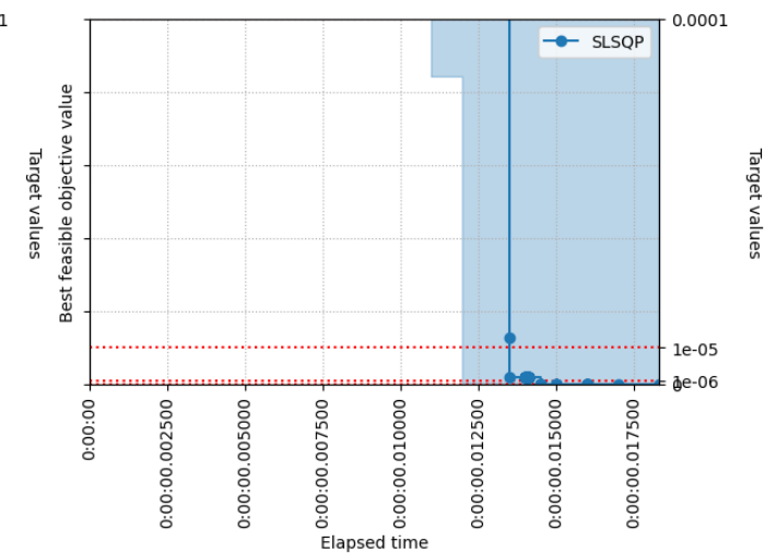
The best feasible objective value of group SLSQP for problem configuration Rosenbrock 5D.
