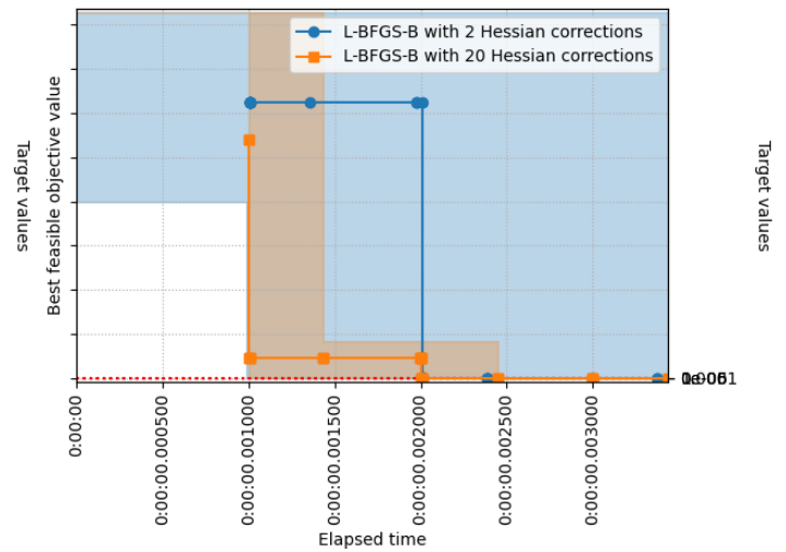
The best feasible objective value of group L-BFGS-B configurations for problem configuration Rastrigin.
