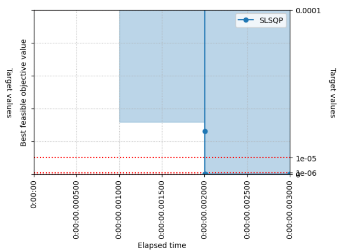
The best feasible objective value of group SLSQP for problem configuration Rastrigin.
