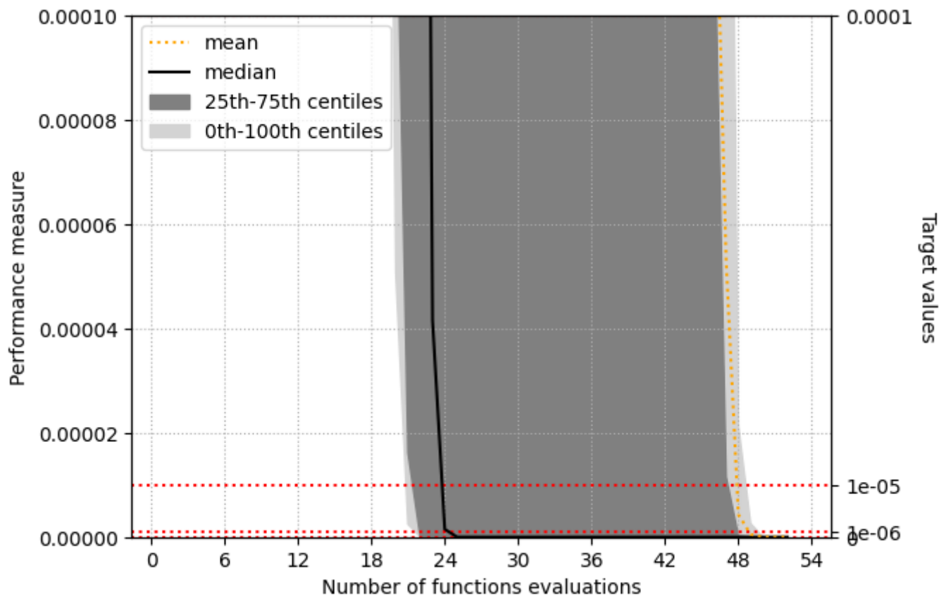
The performance measure of algorithm configuration 'L-BFGS-B with 20 Hessian corrections' for problem 'Rosenbrock'.
