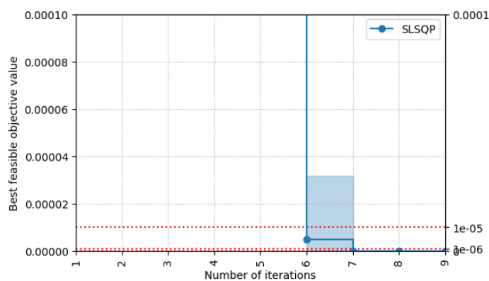
The best feasible objective value of group SLSQP for problem configuration Rastrigin.
