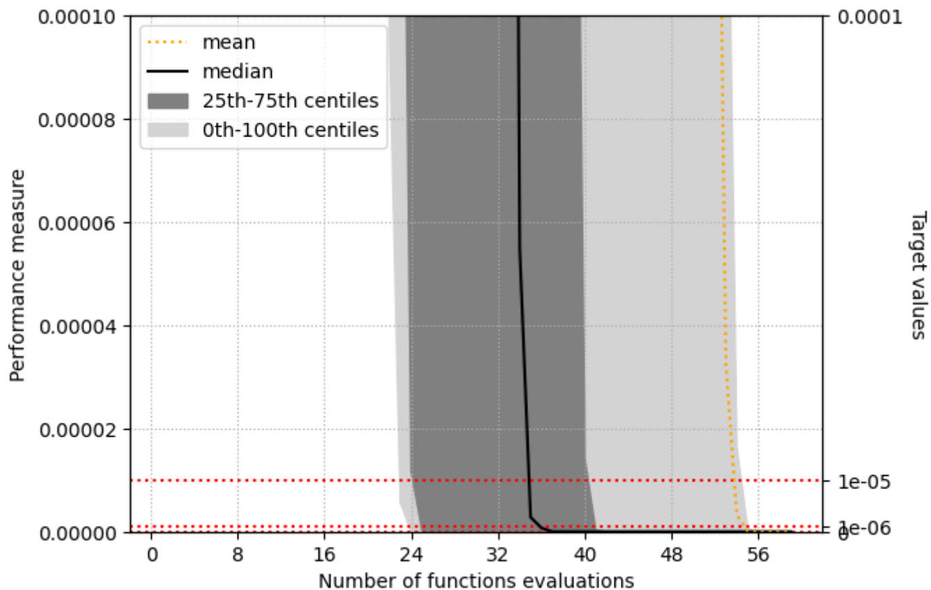
The performance measure of algorithm configuration 'SLSQP' for problem 'Rosenbrock'.
