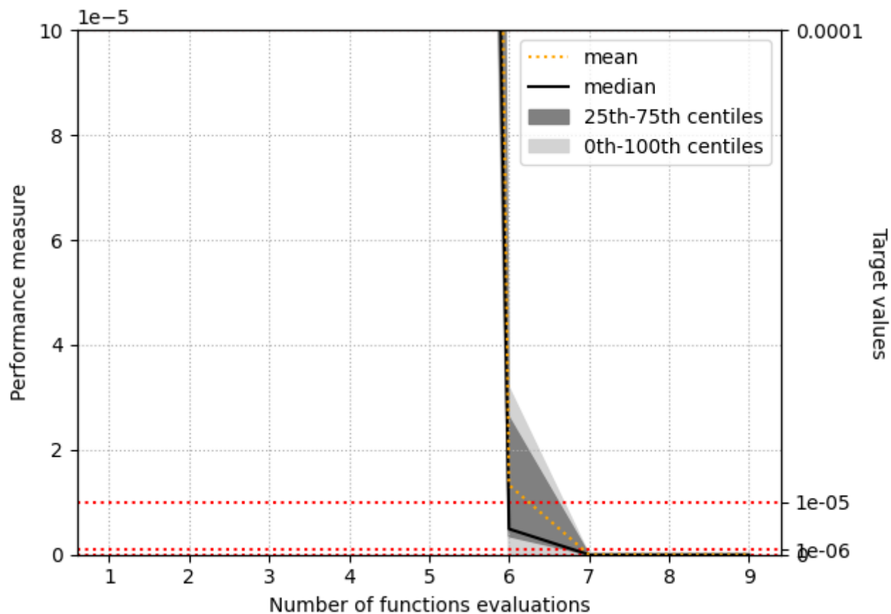
The performance measure of algorithm configuration 'SLSQP' for problem 'Rastrigin'.
