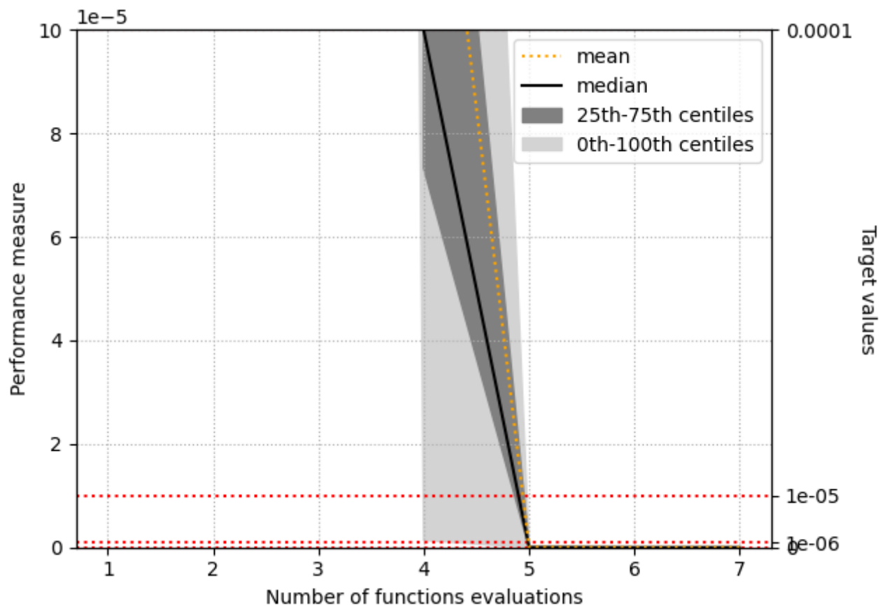
The performance measure of algorithm configuration 'L-BFGS-B with 2 Hessian corrections' for problem 'Rastrigin'.
