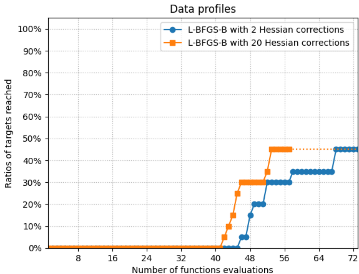
The data profiles of group L-BFGS-B configurations for problem configuration Rosenbrock 5D.
