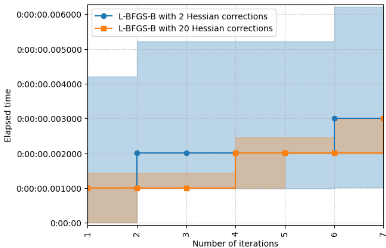
The execution time of group L-BFGS-B configurations for problem configuration Rastrigin.
