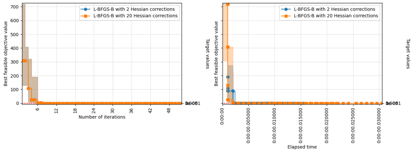
The best feasible objective value of group L-BFGS-B configurations for problem configuration Rosenbrock.
