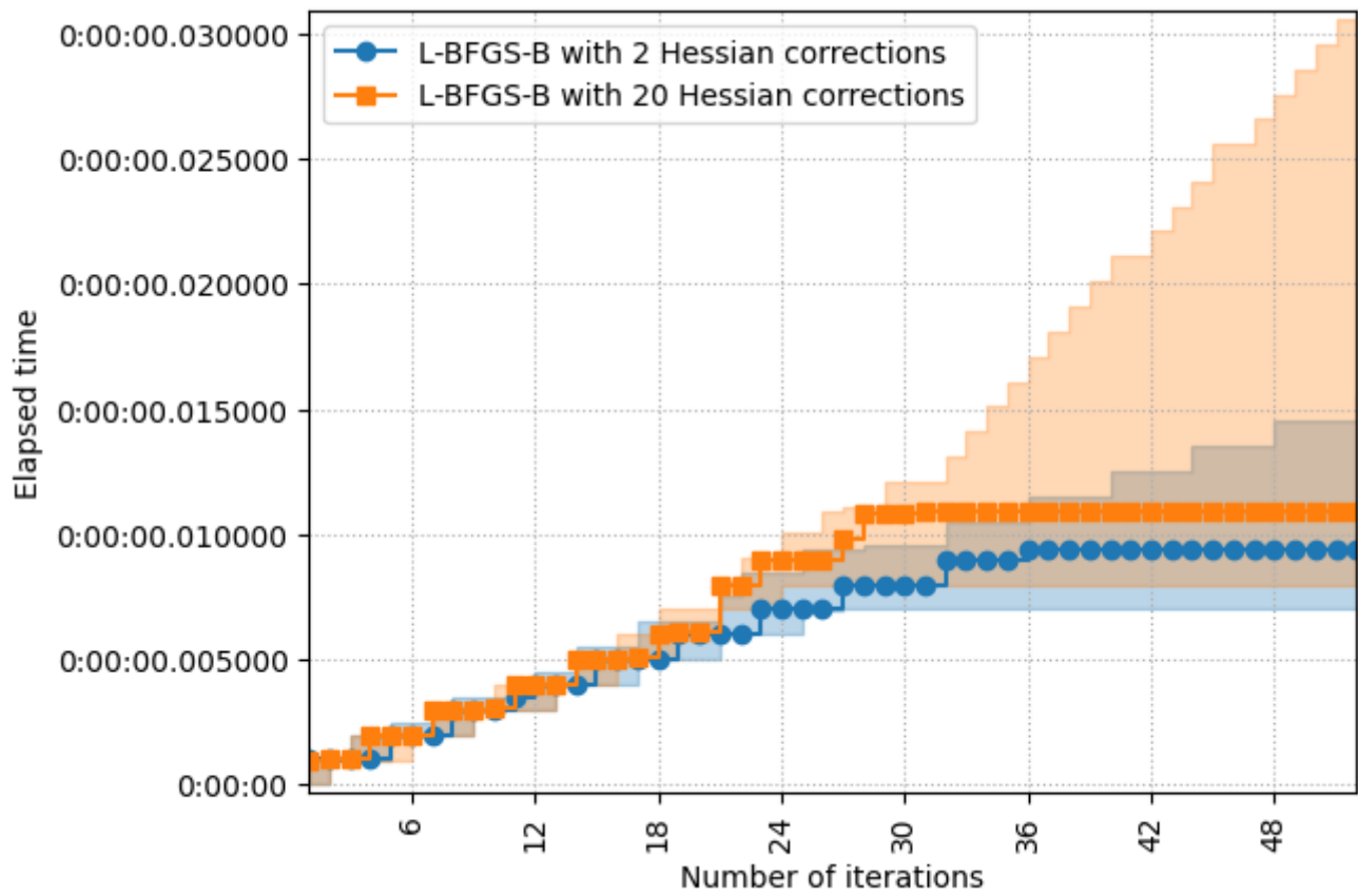
The execution time of group L-BFGS-B configurations for problem configuration Rosenbrock.
