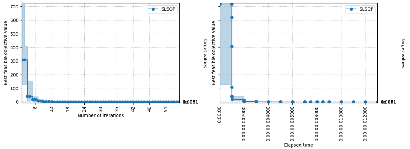
The best feasible objective value of group SLSQP for problem configuration Rosenbrock.
