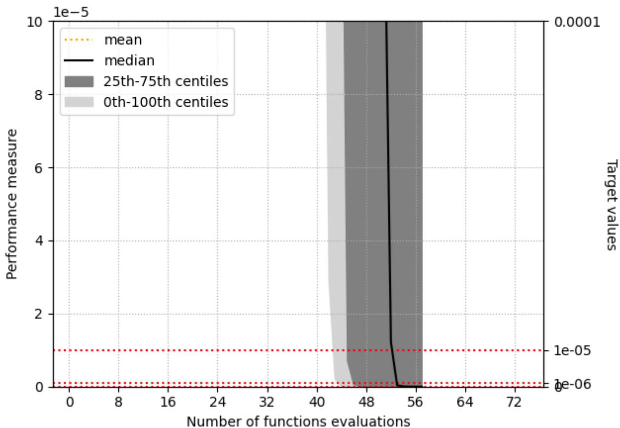
The performance measure of algorithm configuration 'L-BFGS-B with 20 Hessian corrections' for problem 'Rosenbrock 5D'.
