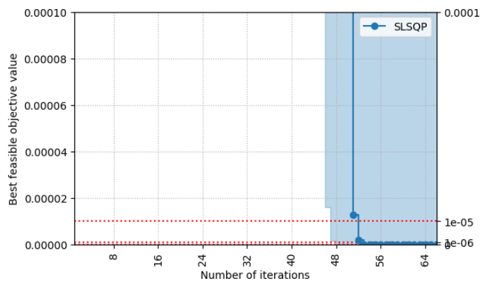
The best feasible objective value of group SLSQP for problem configuration Rosenbrock 5D.
