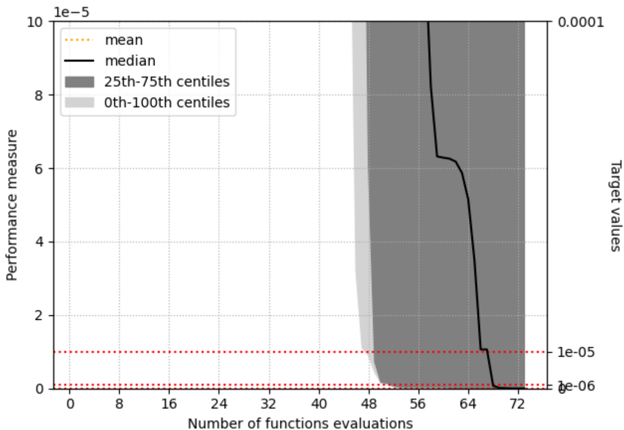
The performance measure of algorithm configuration 'L-BFGS-B with 2 Hessian corrections' for problem 'Rosenbrock 5D'.
