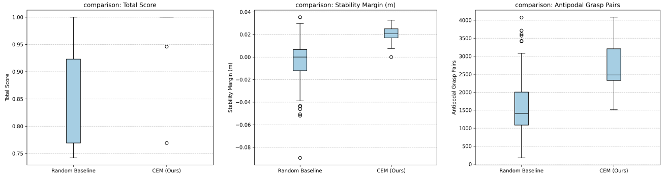
Fig. 5. Per-method distributions over 100 generated objects. The total-suitability panel (left) saturates by design — it is the training objective. Discriminating signal lives in the stability margin (center) and antipodal-pair count (right).
