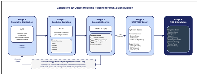
Fig. 3. System pipeline. Offline generation produces a manifest of URDF/SDF assets; the generated_objects_eval ROS 2 package consumes that manifest from MoveIt 2 and Gazebo nodes.
