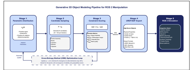
Fig. 2. System Pipeline: From parametric distribution to ROS 2 simulation.
