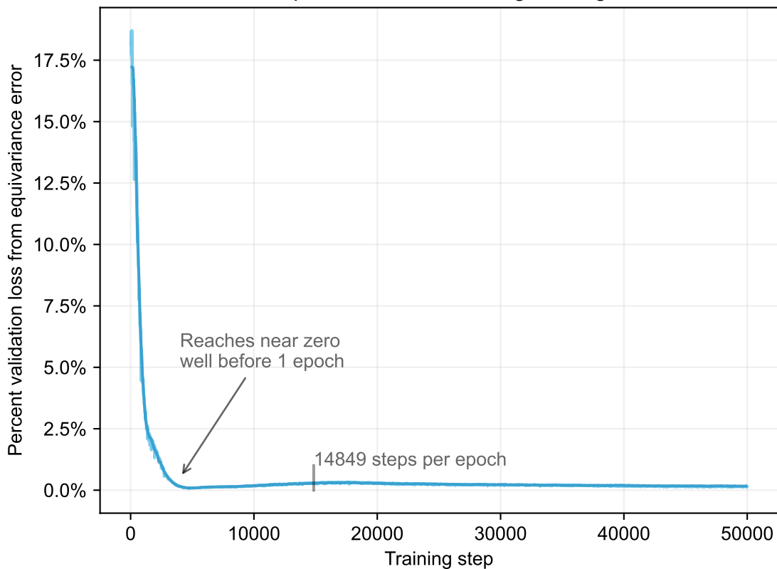
Equivariance error during training
