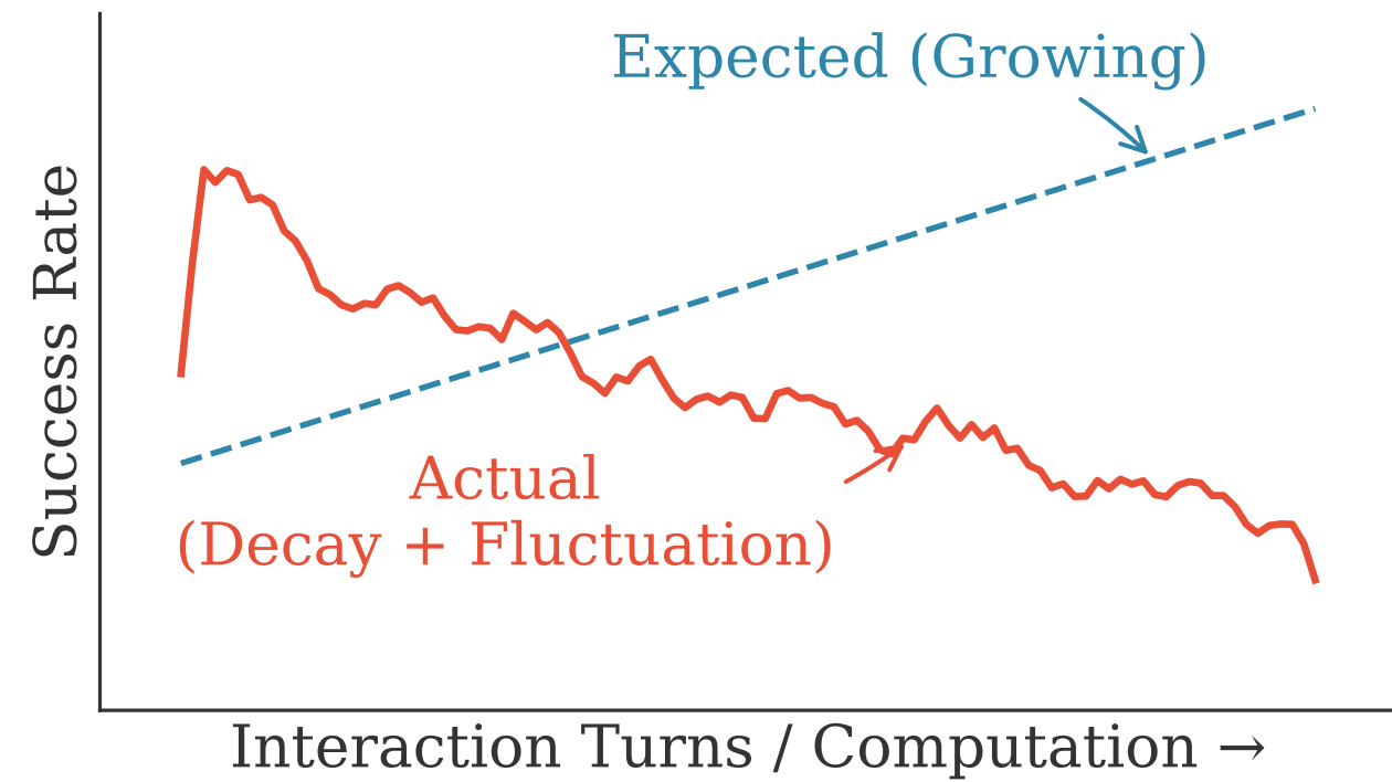
B. Agentic Sequential Scaling Trend
