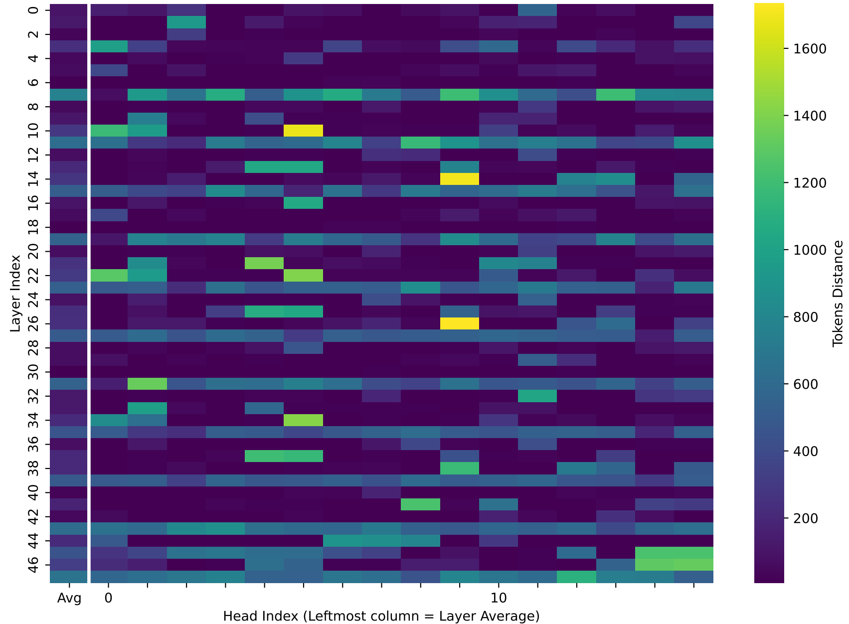
A. Mean Attention Distance (Layer vs Head)
