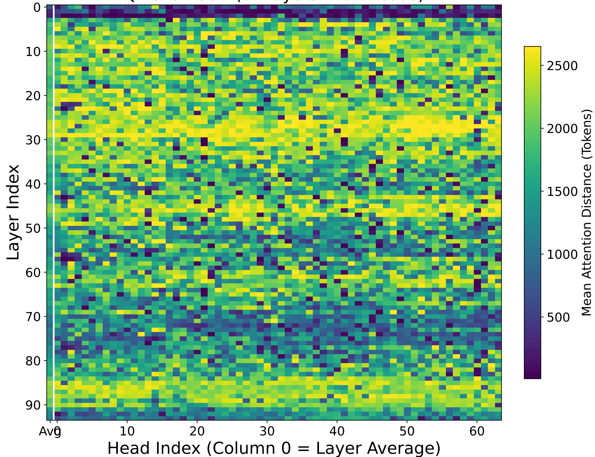
Qwen3-235B (94 layers × 64 heads)
