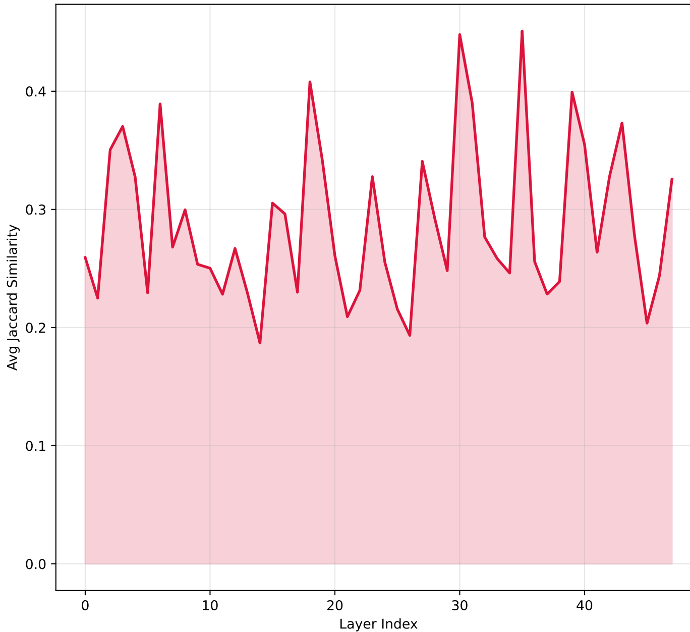
B. Head Redundancy (Intra-layer Overlap)
