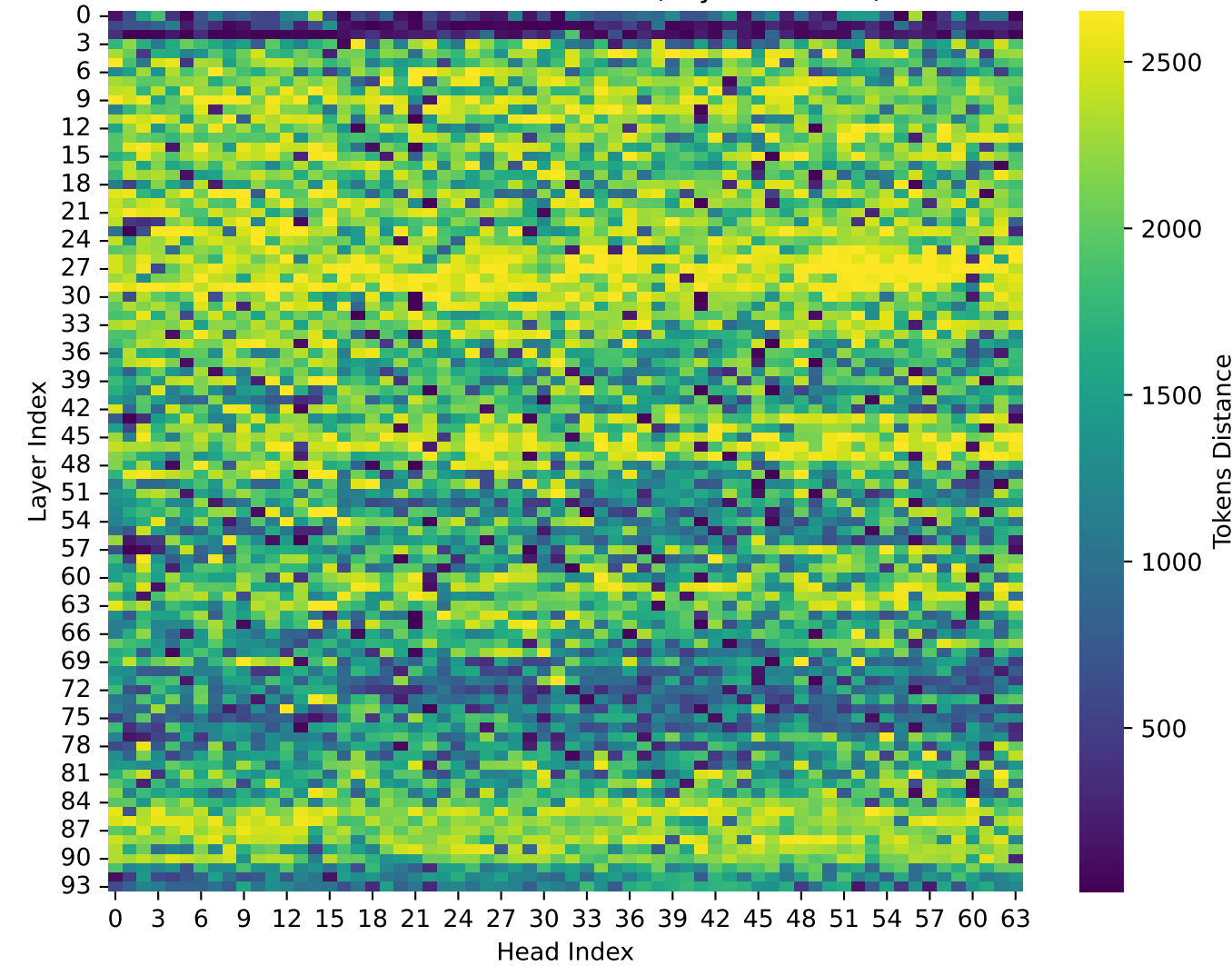
A. Mean Attention Distance (Layer vs Head)
