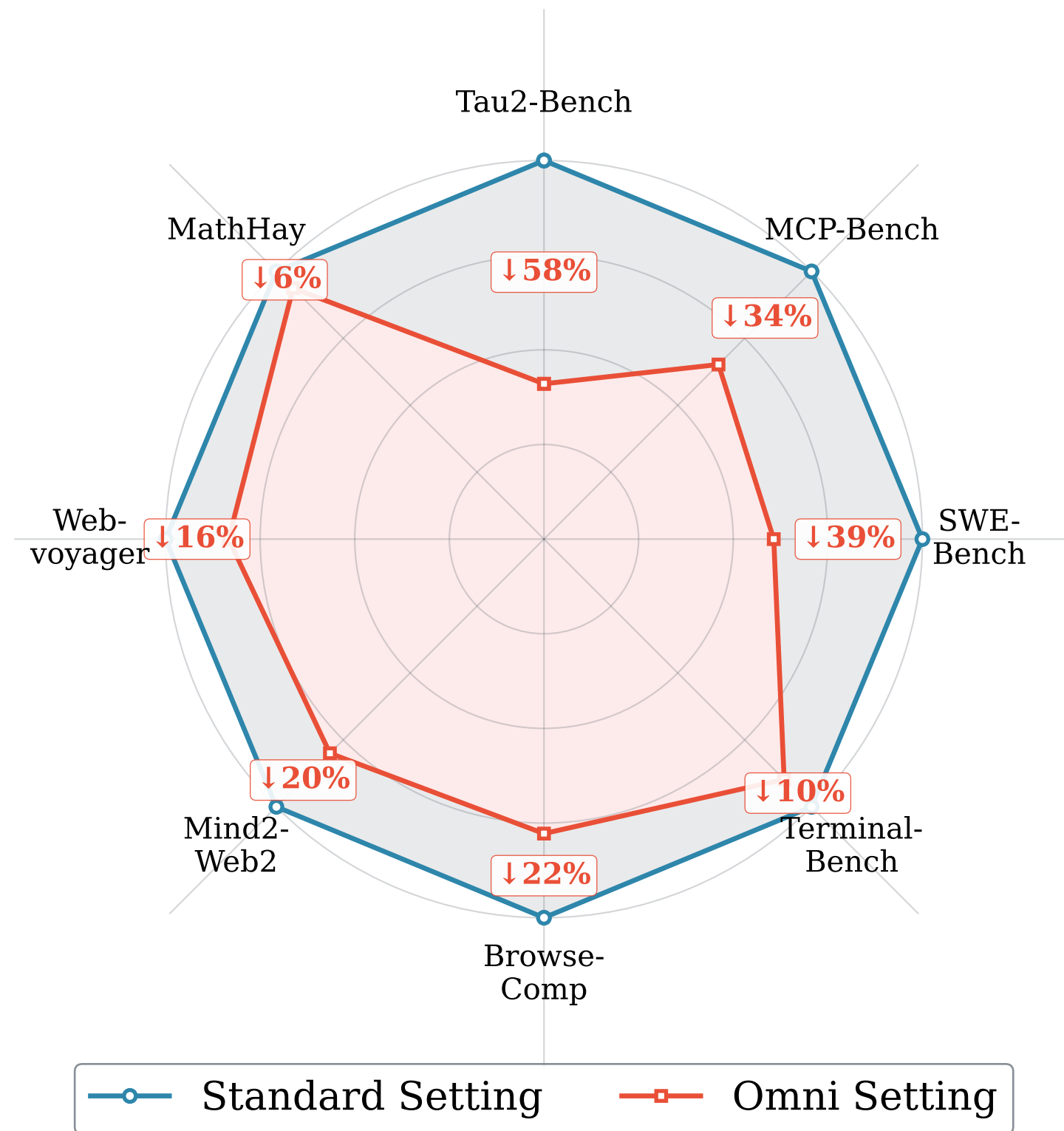
A. Performance Degradation: Simplified → Real-world Settings
