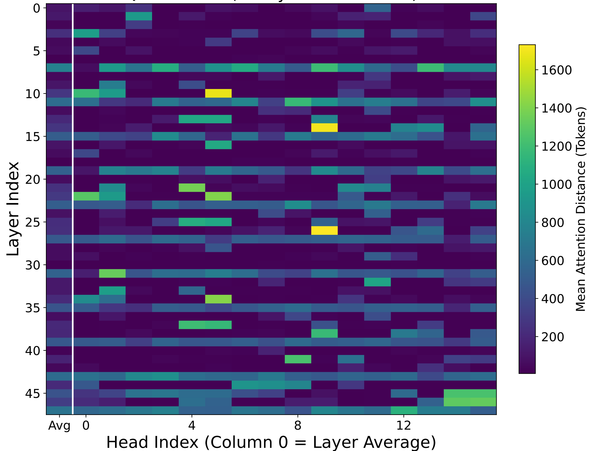
Qwen3-Next (48 layers × 16 heads)
