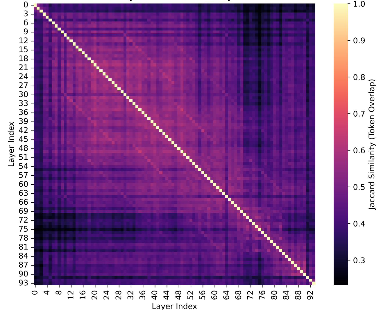
C. Inter-layer Token Consistency Matrix
