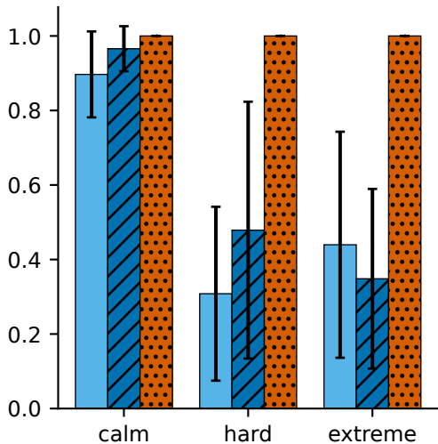
Deflated Sharpe (sign policy)
