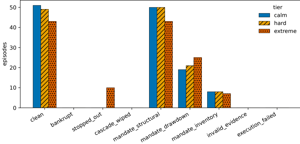
Figure 13: Failure-mode counts per tier, each summed over the 8 policies and 16 seeds (128 episodes per tier, 384 in total), for every disposition in the rollup schema; the bankruptcy, cascade-wipe, invalid-evidence and execution-failure bars are zero. Tiers differ by colour and by hatching (Calm plain, Hard diagonal, Extreme dotted).
