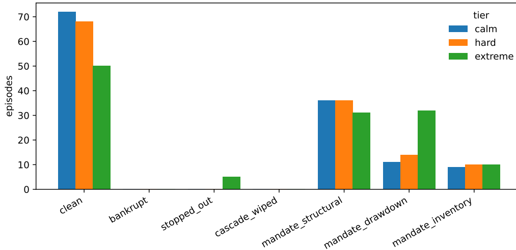
Figure 15: Failure-mode distribution per tier per policy over 384 classified episodes.
