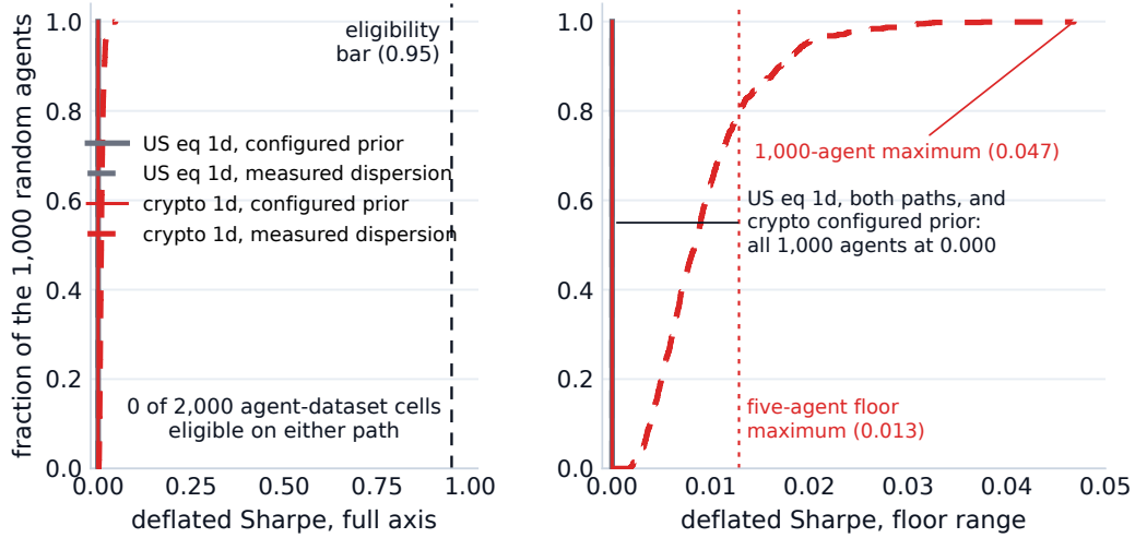
Figure 3: Empirical distribution of the deflated Sharpe over the 1,000 random agents on each daily dataset, under the configured prior and under field-measured dispersion, computed from the committed thousand-agent records. Left: the full axis with the \beta = 0.95 eligibility bar; every curve is pinned at the origin, and none of the 2,000 agent-dataset cells is eligible on either path. Right: the same curves on the range the floor occupies. Daily US indices sit at 0.000 on both paths, as does daily crypto under the configured prior; daily crypto under measured dispersion reaches 0.047 at its thousand-agent maximum, against 0.013 among the first five agents, which is the shipped five-agent floor.
