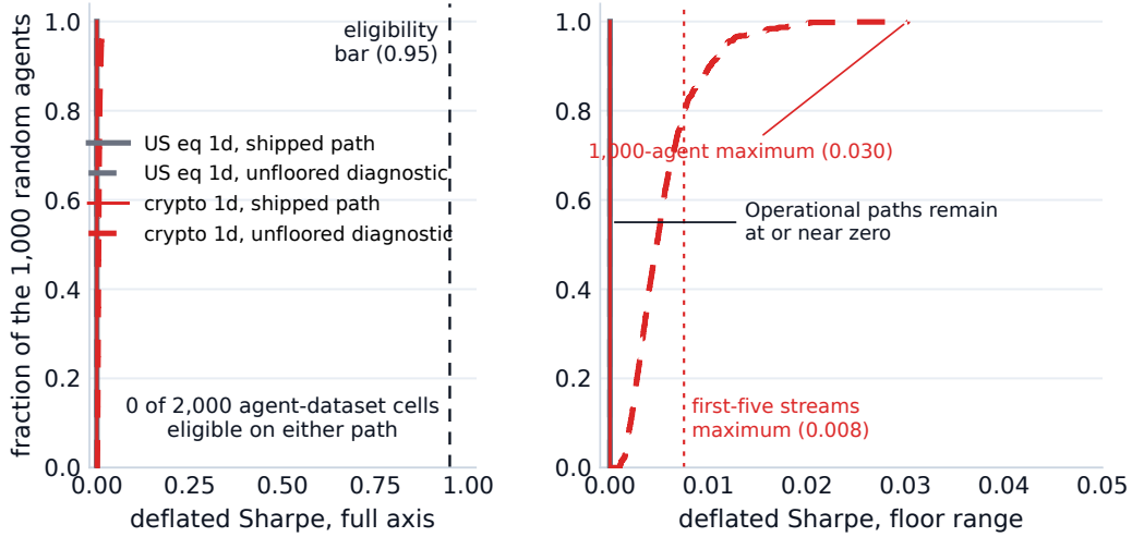
Figure 3: Empirical distributions over the 1,000 random agents on each daily dataset, all scored at the observable 1,000-trial footprint. The solid operational curves apply the shipped annualized dispersion floor; the dashed curves are deliberately unfloored diagnostics. The daily-crypto diagnostic reaches 0.0302, but that value is not used by ranking. Left: the full axis with the \beta = 0.95 bar. Right: the diagnostic range. No agent is eligible, and both operational maxima are zero.
