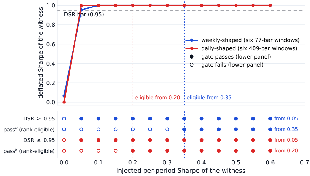
Figure 2: The pass-witness boundary, computed from the committed witness records by the evidence-figure script. Top: the witness’s deflated Sharpe against its injected per-period Sharpe on the two window geometries, with the 0.95 bar; the dotted verticals mark the onset of rank eligibility, 0.35 on the weekly geometry and 0.20 on the daily. Bottom: the two gate outcomes at every injected edge, filled where the gate passes. DSR clears from the first nonzero sampled edge, s = 0.05 , on both geometries, so \text{pass}^k alone binds everywhere on this sweep: it turns on at 0.20 daily and 0.35 weekly, which are the onsets marked above.
