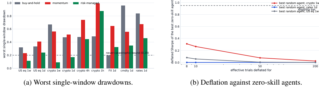
Figure 4: Computed from the committed evidence records by a committed script. (a) The risk-managed agent posts the smallest worst-window drawdown of any trading agent on seven of nine datasets, while both long-only references breach the 20 percent per-regime bound almost everywhere and hourly momentum loses 99.3 percent in one window; the two exceptions, hourly crypto and daily FX, are where the trend filter itself whipsaws. (b) The best zero-skill agent’s operational DSR as the effective trial count grows. A host setting of one becomes eight because the submitted field has eight streams; the measured dispersion is also bounded below by the annualized prior. The curve therefore describes the shipped ranking path, not an unfloored diagnostic.
