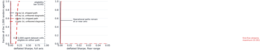
Figure 3: Empirical distributions over the 1,000 random agents on each daily dataset, all scored at the observable 1,000-trial footprint. The solid operational curves apply the shipped annualized dispersion floor; the dashed curves are deliberately unfloored diagnostics. The daily-crypto diagnostic reaches 0.2500, but that value is not used by ranking; its operational maximum is 0.0012. Left: the full axis with the \beta = 0.95 bar. Right: the diagnostic range. No agent is eligible.
