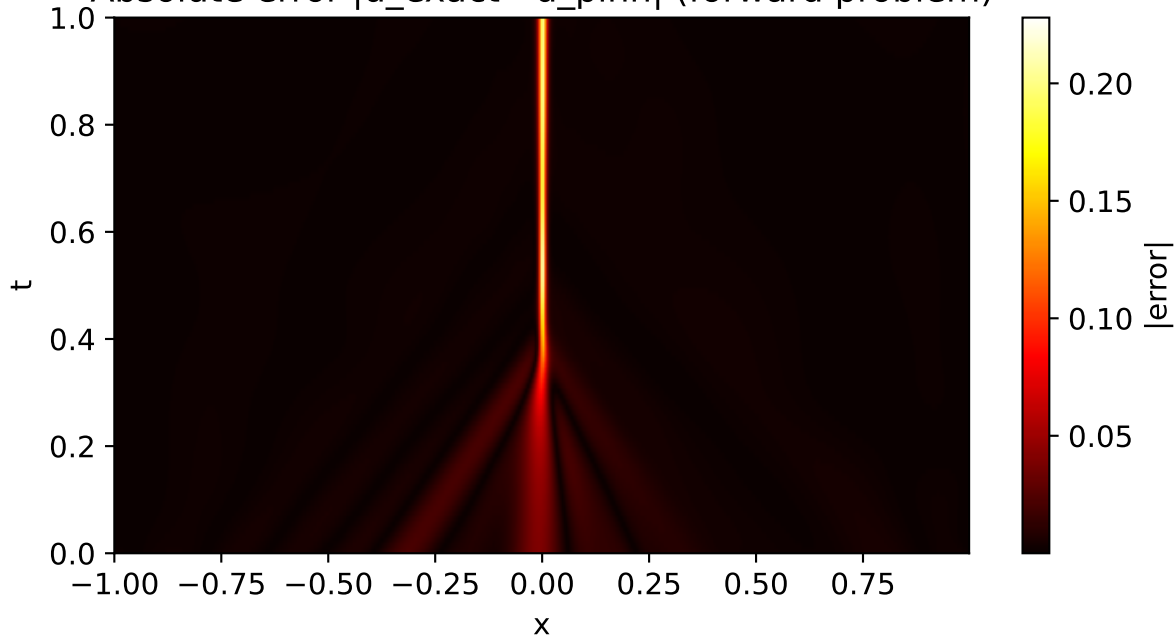
Absolute error |u_{\text{exact}} - u_{\text{pinn}}| (forward problem)
