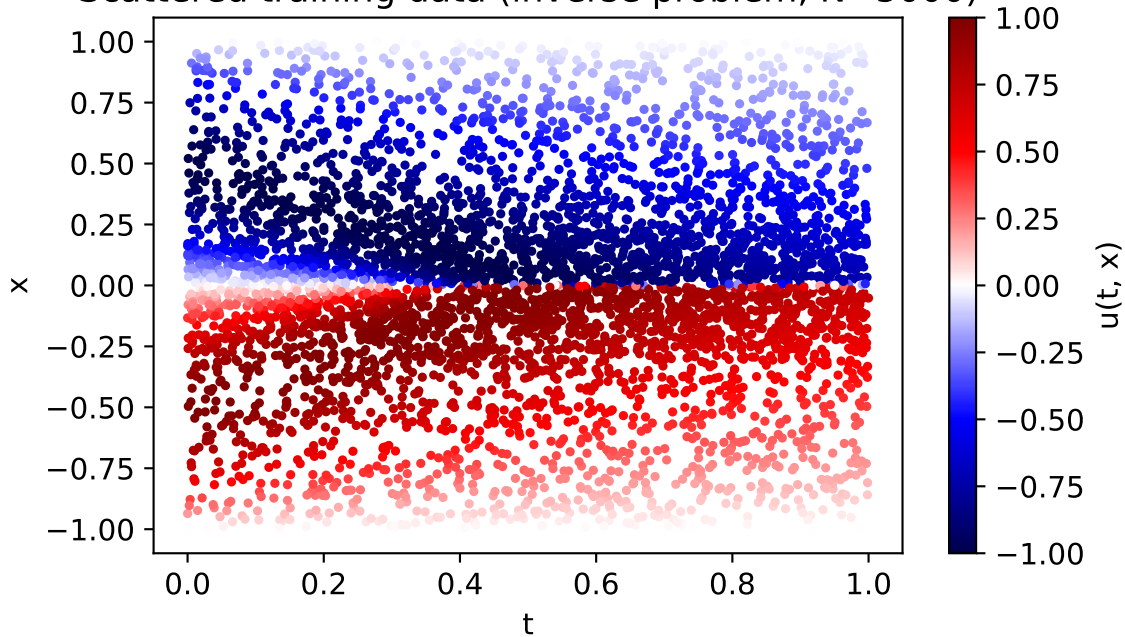
Scattered training data (inverse problem, N=5000 )
