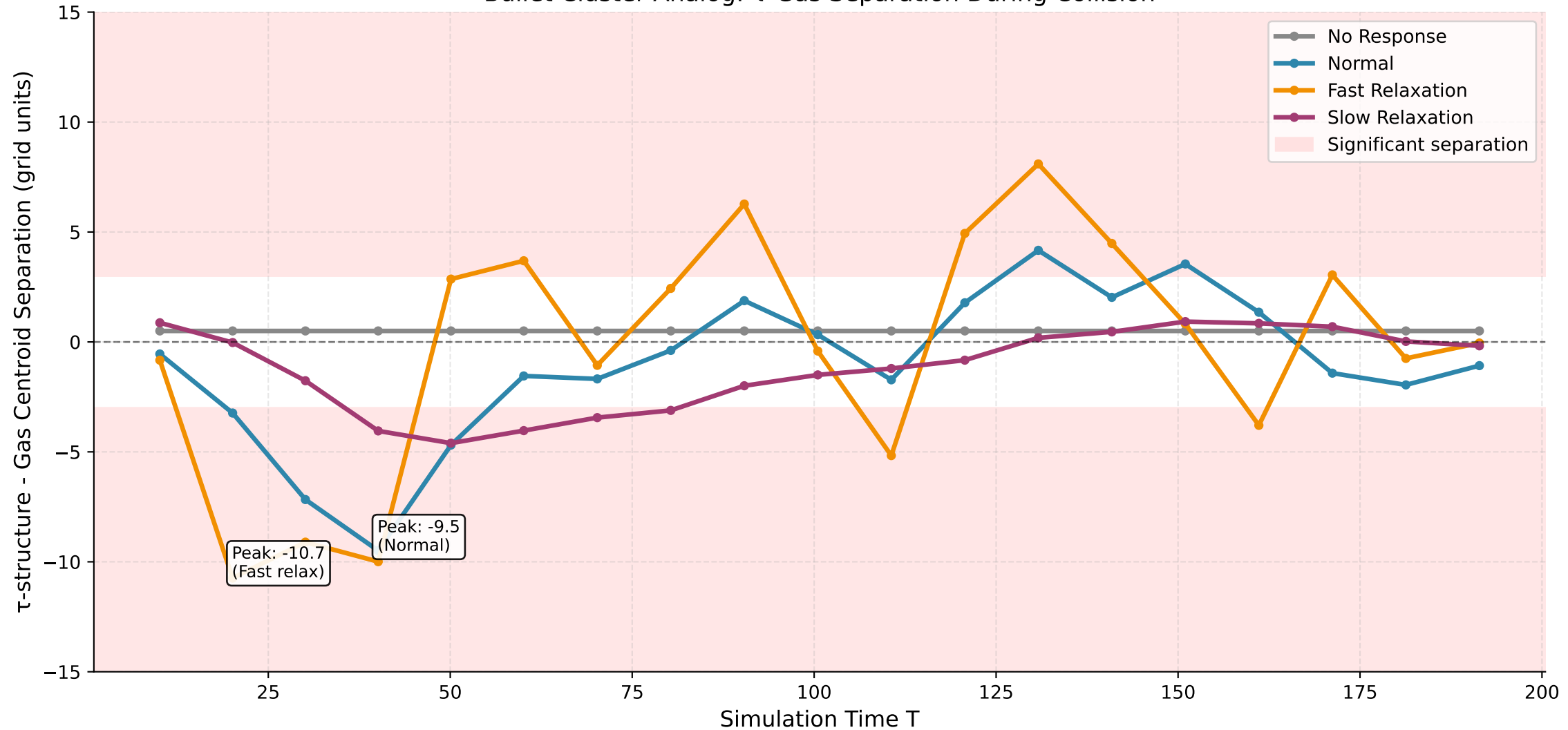
Bullet Cluster Analog: \tau -Gas Separation During Collision
