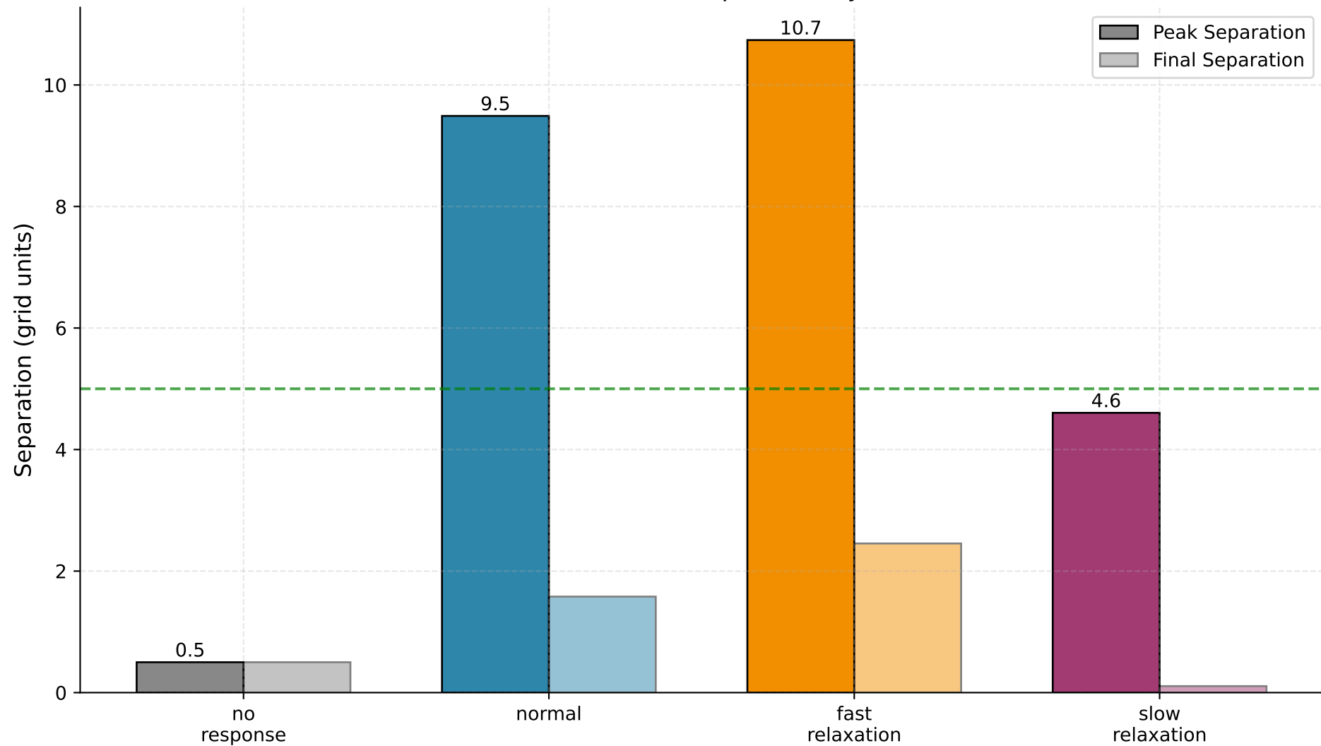
Peak vs Final \tau -Gas Separation by Variant
