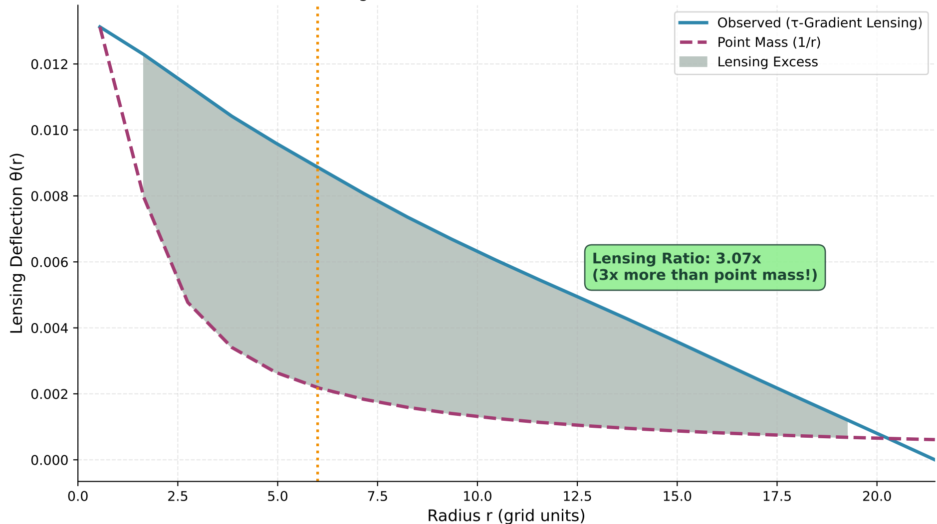
Lensing Profile: \tau -Gradient Effect vs Point Mass
