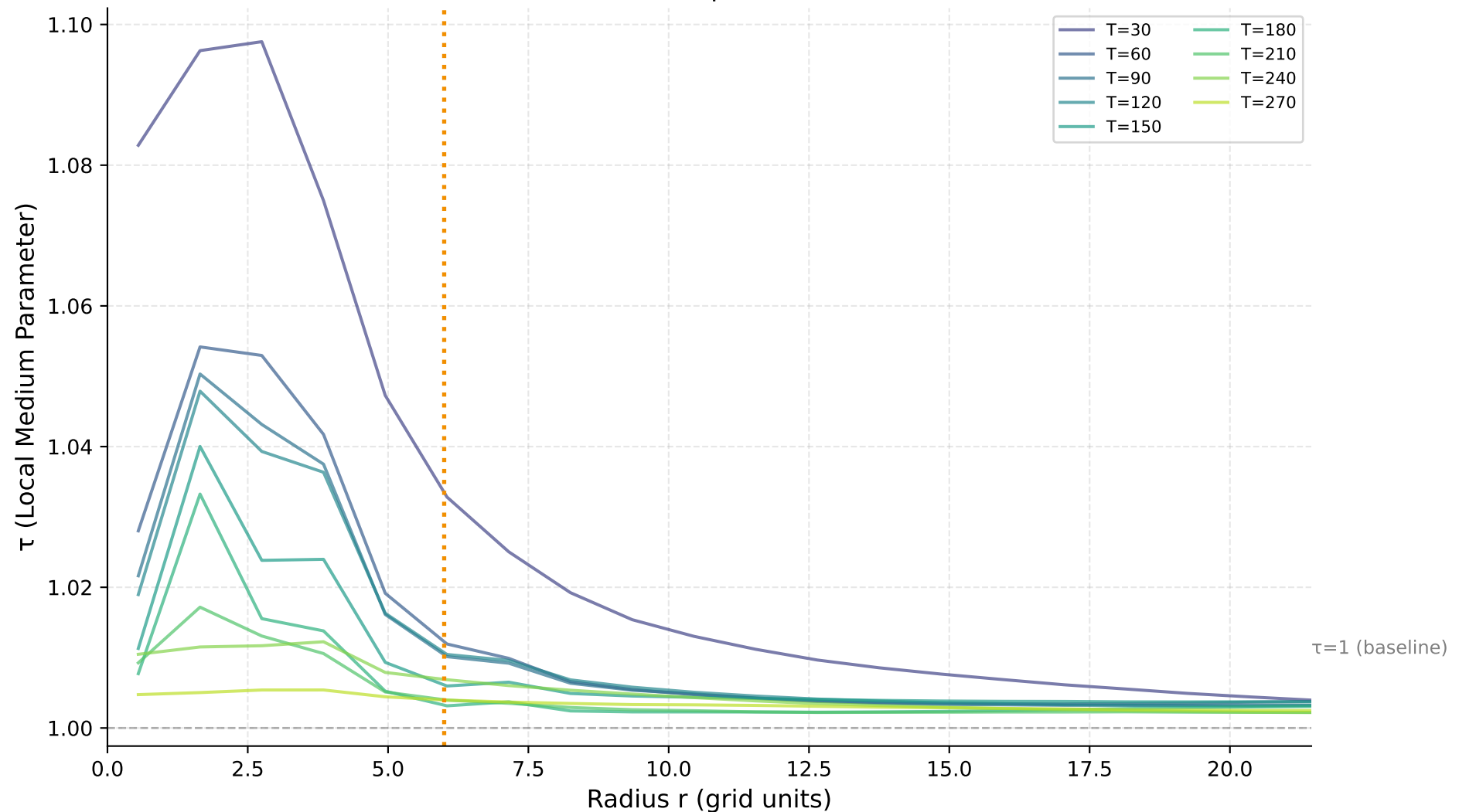
\tau Profile Evolution: Medium Response to Central Concentration
