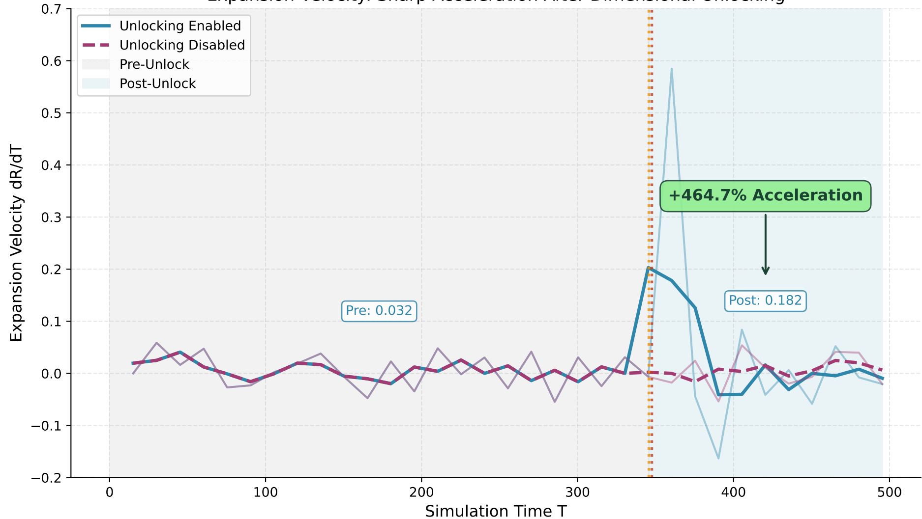
Expansion Velocity: Sharp Acceleration After Dimensional Unlocking
