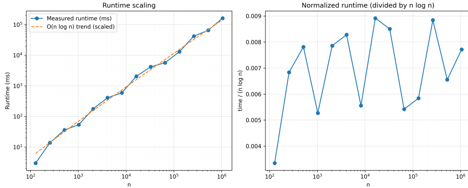
Figure 9: Runtime scaling on structured CETSP instances with linear tour size. The O(n \log n) trend fits the measured data closely.
