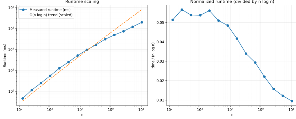
Figure 8: Runtime scaling on random CETSP instances. Runtime grows slower than O(n \log n) due to sublinear growth of the tour size.
