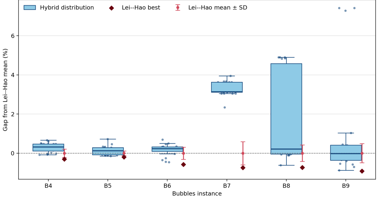
Figure 7: Run distributions for the nontrivial Bubbles instances, expressed relative to Lei and Hao’s reported mean. Points show the 20 runs; boxes show their quartiles. The high variance on bubbles8 and bubbles9 contrasts with the persistent gap on bubbles7 .
