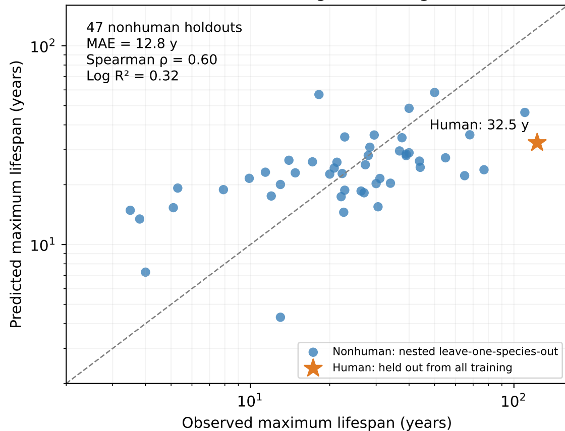
FDR-selected genes + ridge
