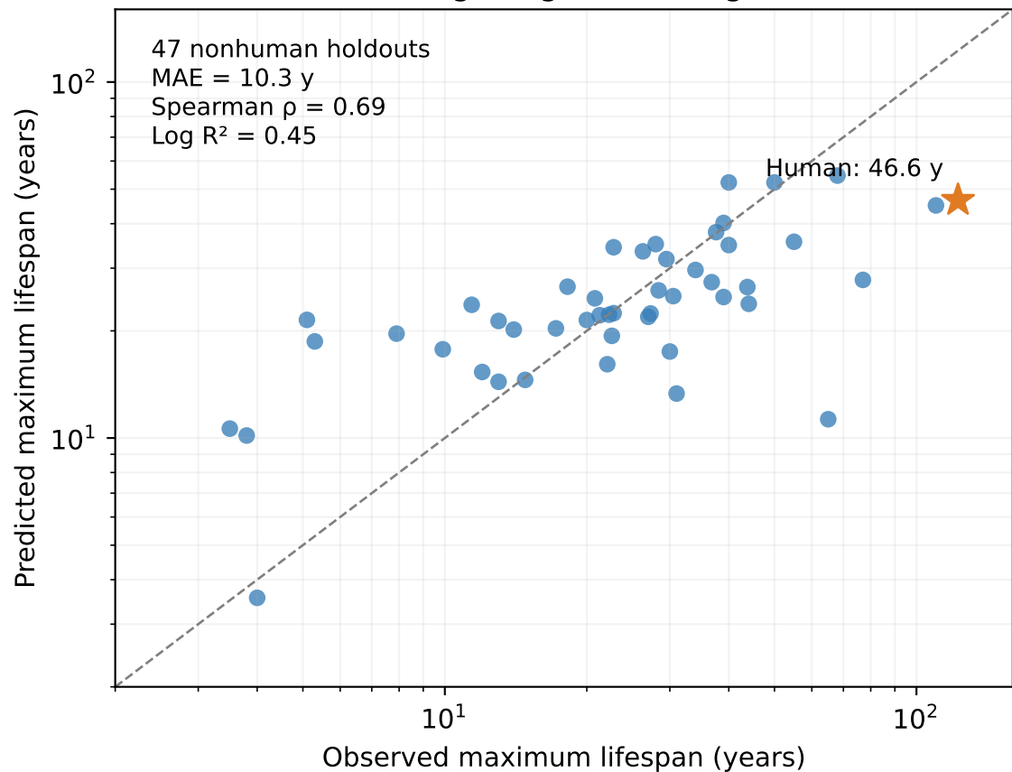
All eligible genes + ridge
