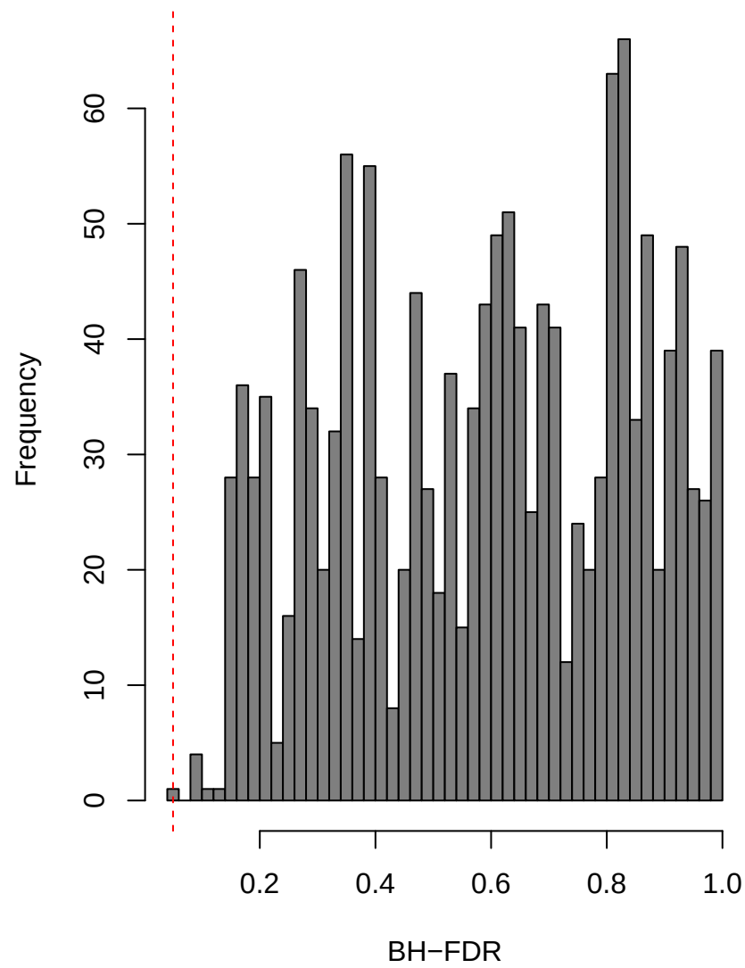
B. Pure 2-df interaction P
