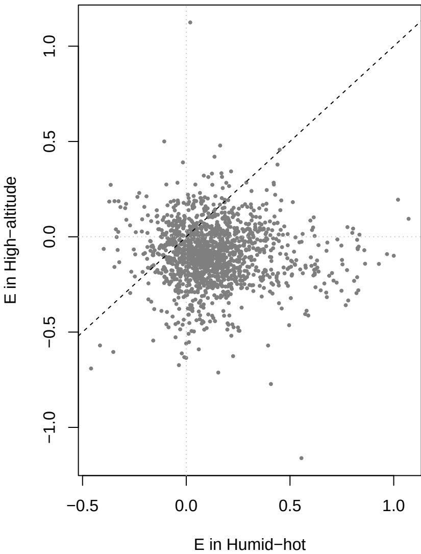
A. Environment-stratified E
