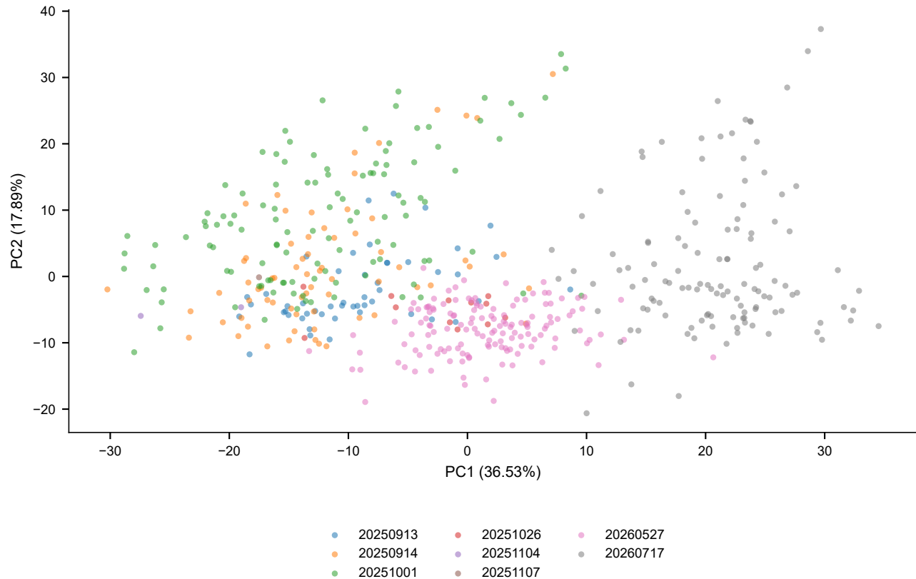
Complete-case PCA by MS batch proxy
