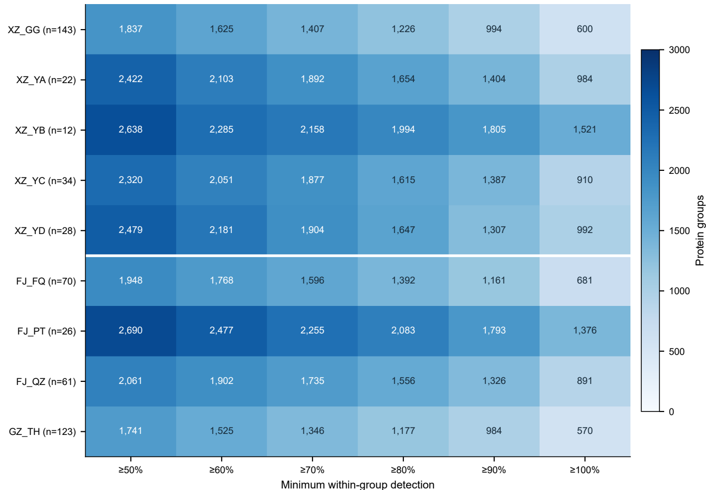
Group-level protein coverage across detection thresholds
