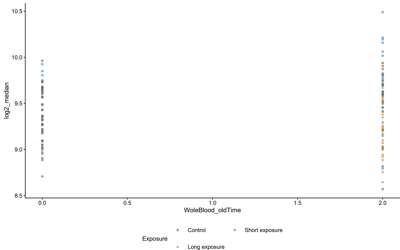
WoleBlood_oldTime and log2_median
