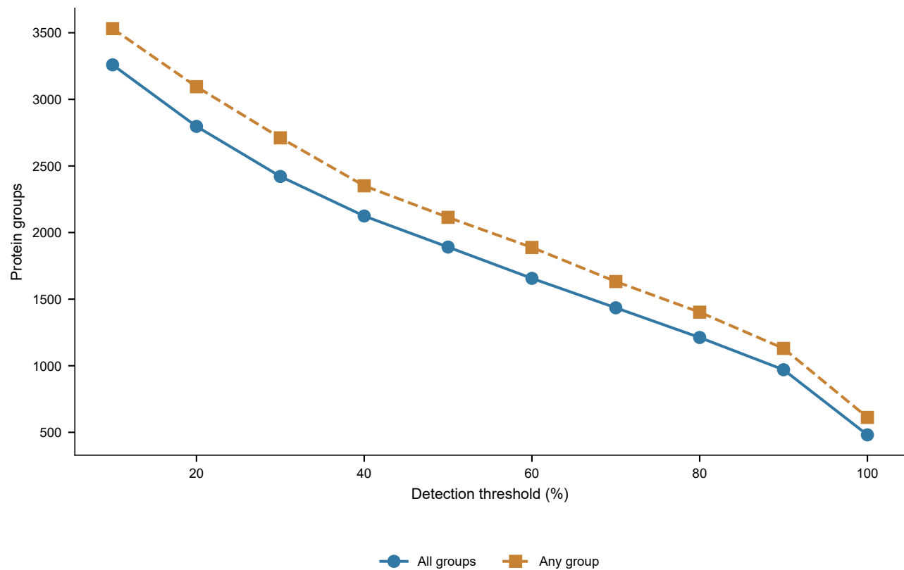
Shared protein coverage across environments
