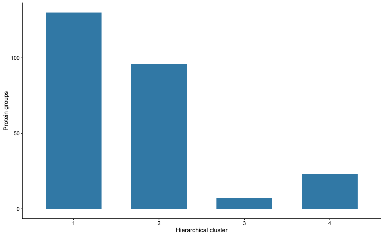
Exploratory hierarchical cluster sizes (K = 4)
