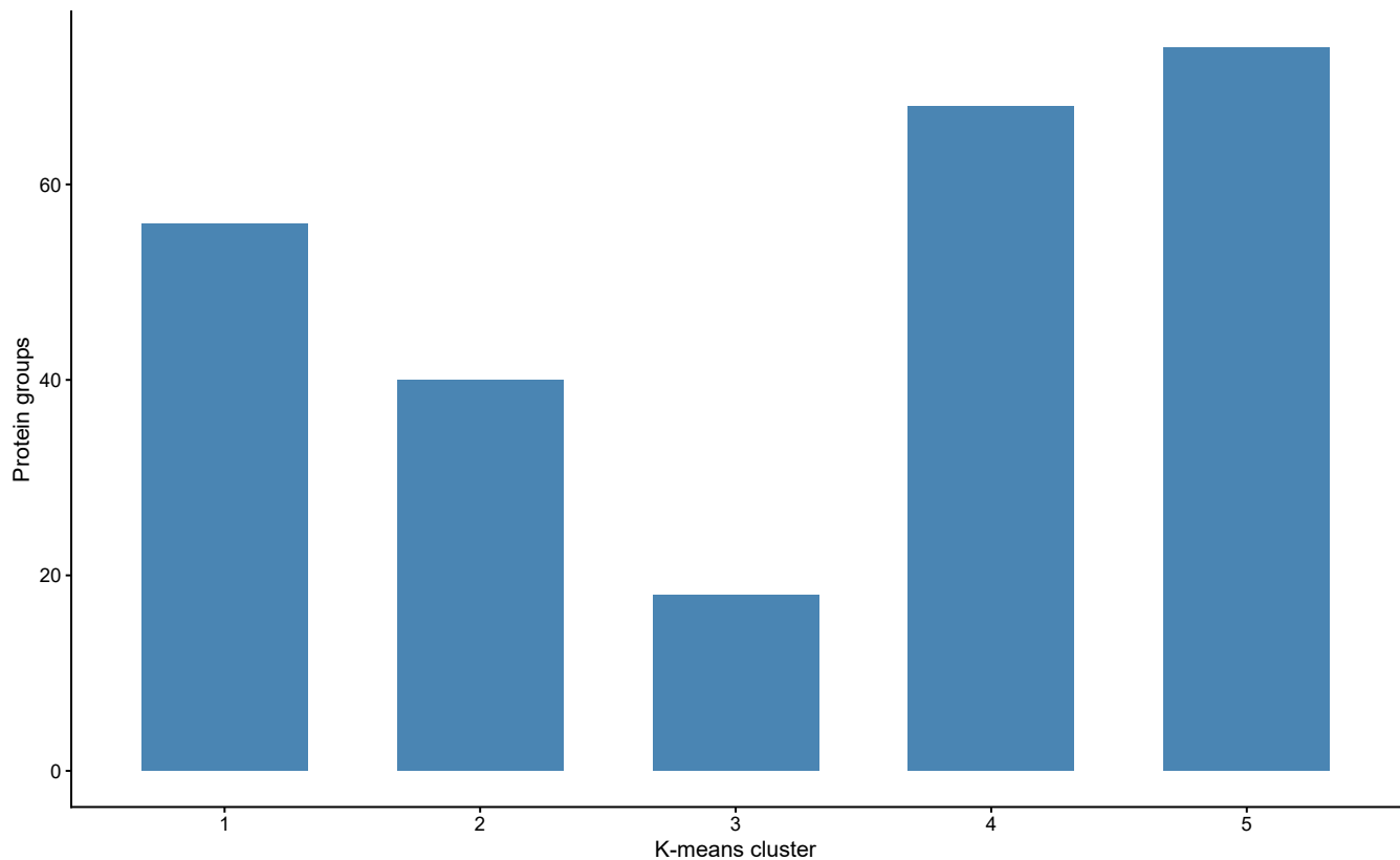
Exploratory K-means sensitivity: K = 5
