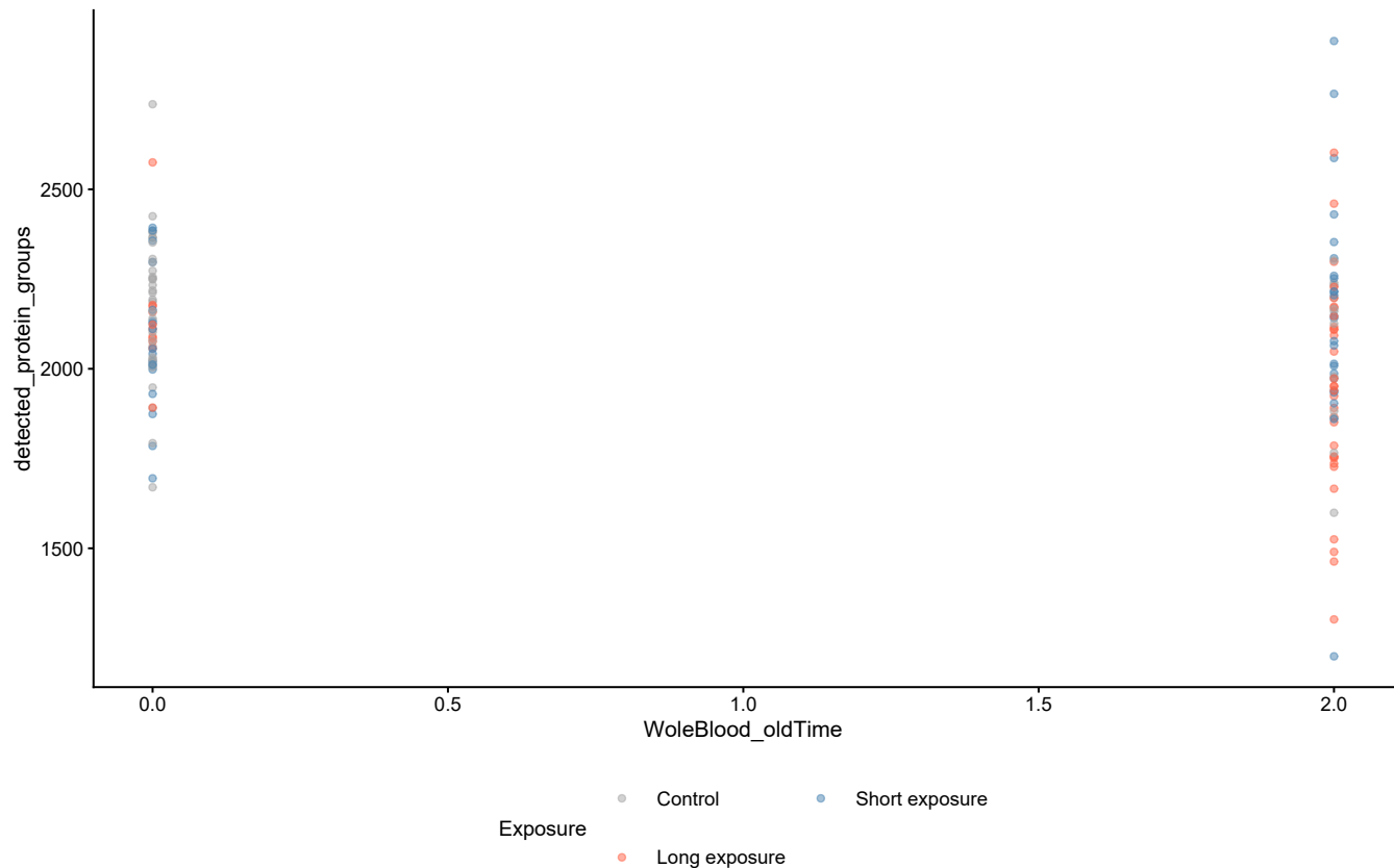
WoleBlood_oldTime and detected_protein_groups
