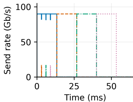
Homa
