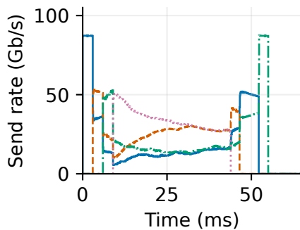
TIMELY
