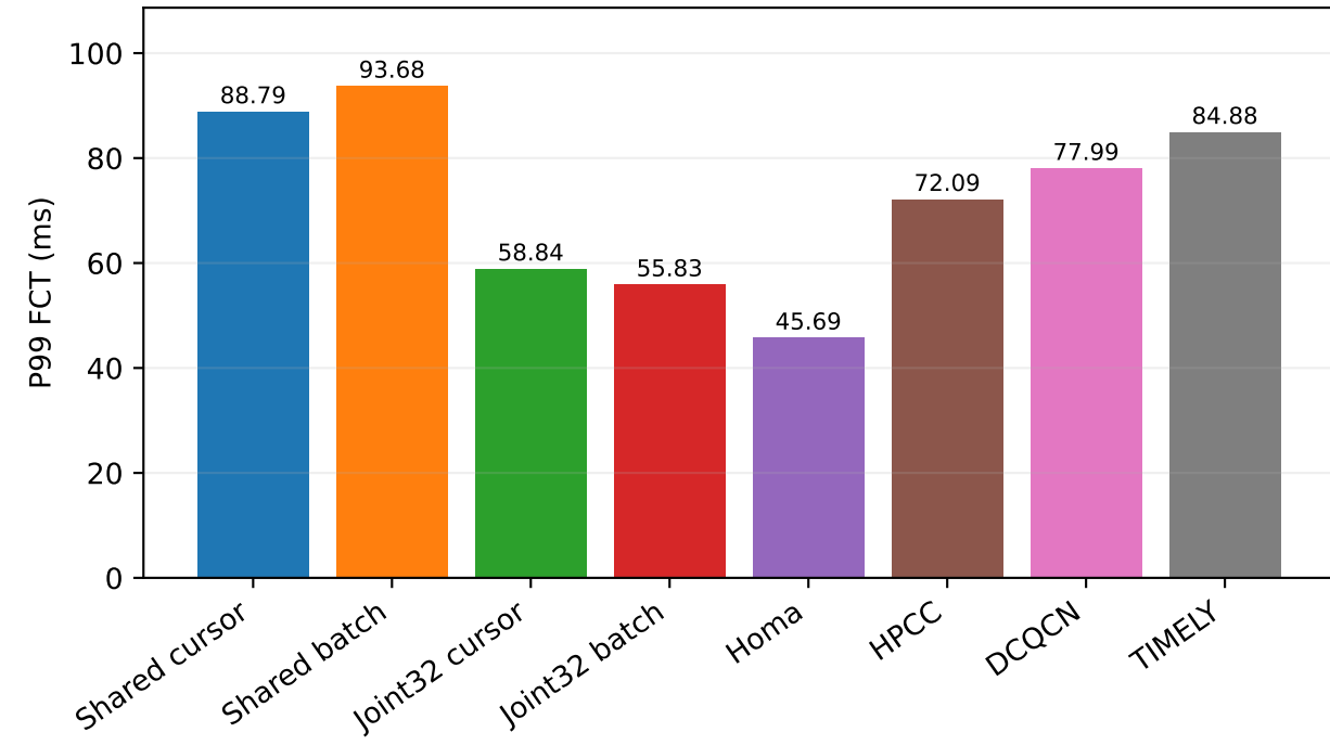
Same-build comparison with all four baselines Full DP2; development seed 301; lower is better
