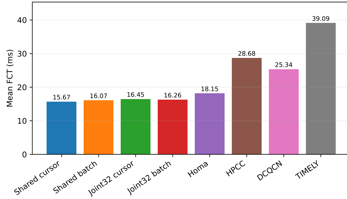
Same-build comparison with all four baselines Full DP2; development seed 301; lower is better
