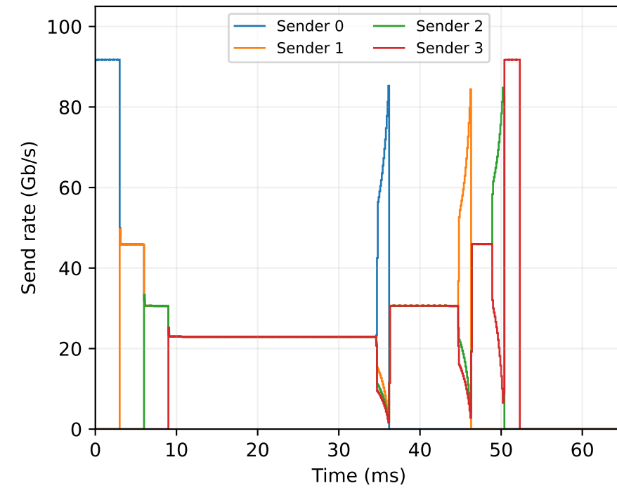
K1: original Jain=1.000000
