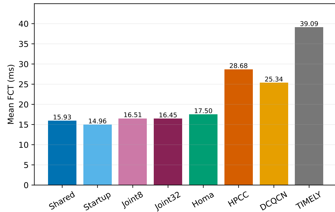
Full DP2; development seed 301; one observation per profile; lower is better
