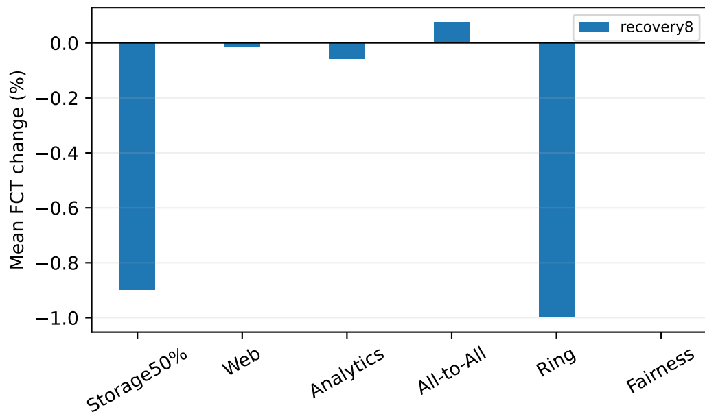
Bounded recovery; relative to same-build Shared; observed seed301; positive=worse
