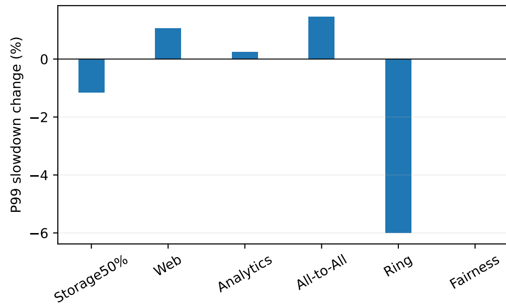
Bounded recovery; relative to same-build Shared; observed seed301; positive=worse
