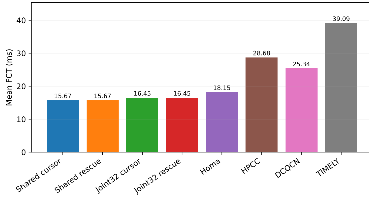
Same-build comparison with all four baselines Full original DP2; development seed 301; lower is better
