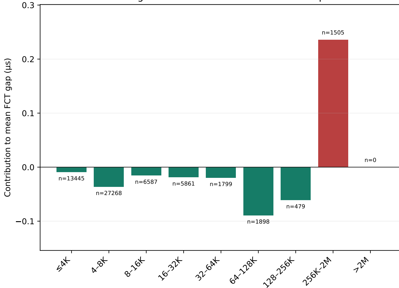
Storage30: total GUARD – Homa = -0.013 \mu s
