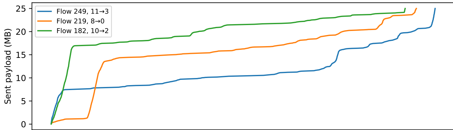
causal_shared_trace; three slowest flows, development seed 301
