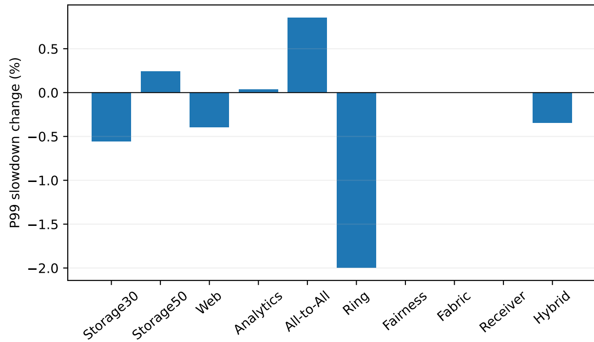
One-base-RTT ACK deadline versus matched Shared; ten original scenes; positive = worse
