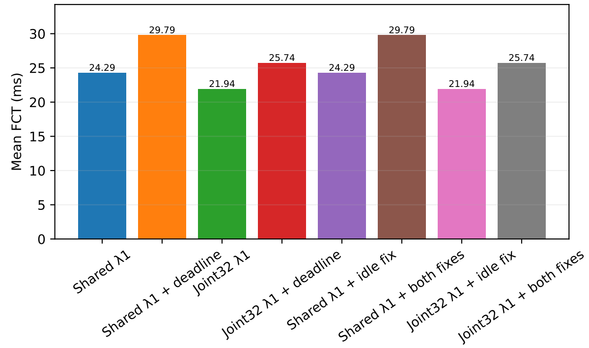
ACK deadline and idle-timer controls (two labeled source revisions); full DP2; development seed 301; lower is better
