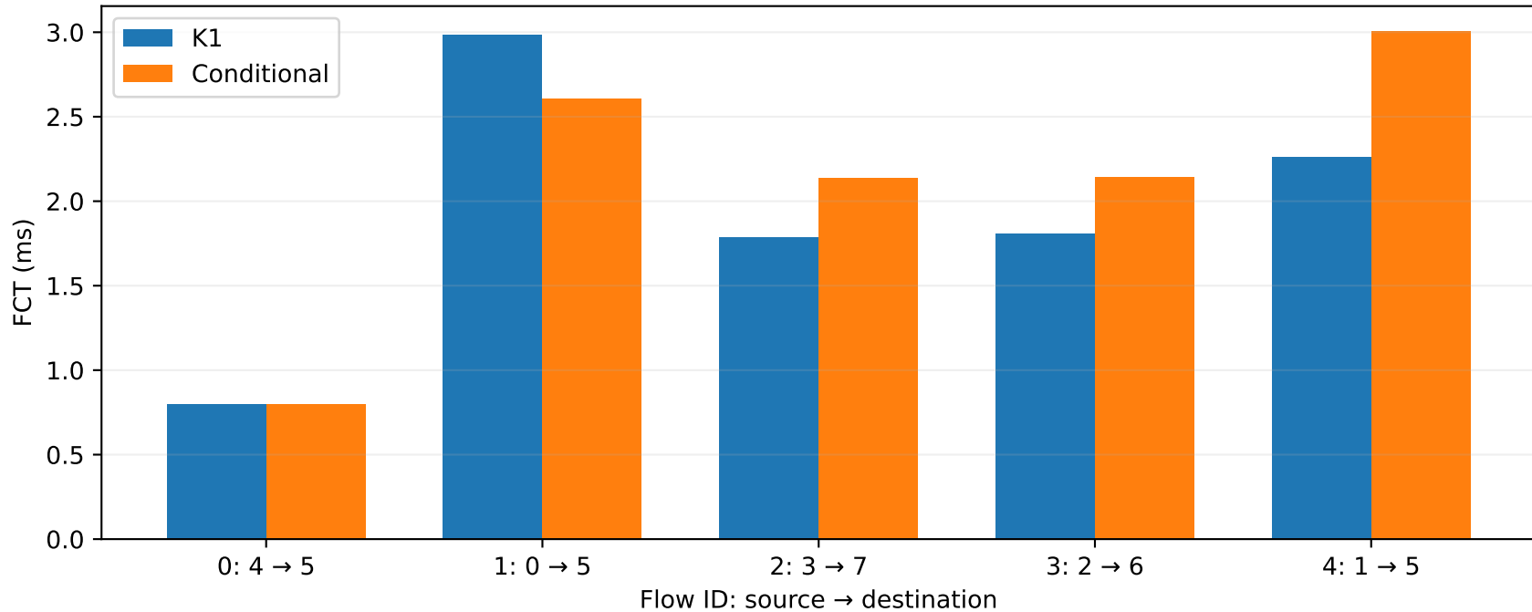
Hybrid: all five original 8 MiB flows, seed 301
