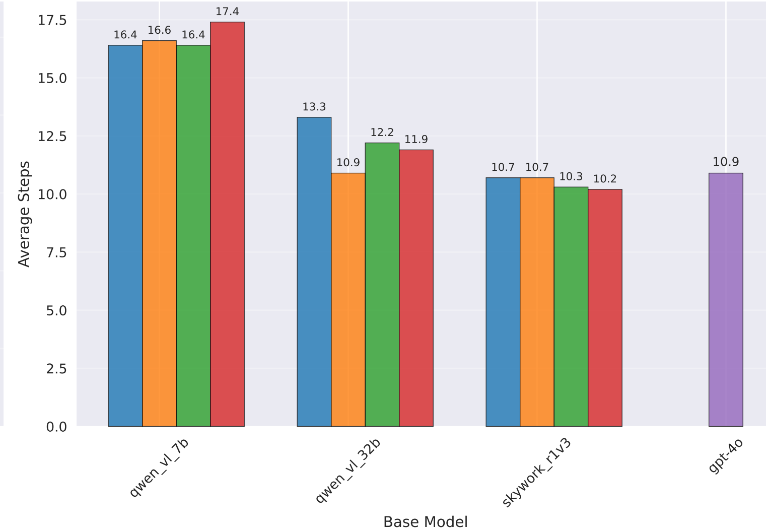
Average Steps Comparison
