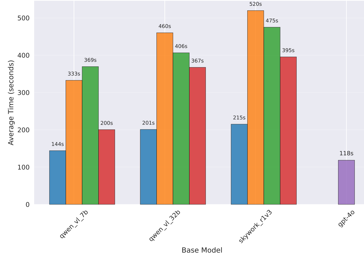
Average Time Comparison
