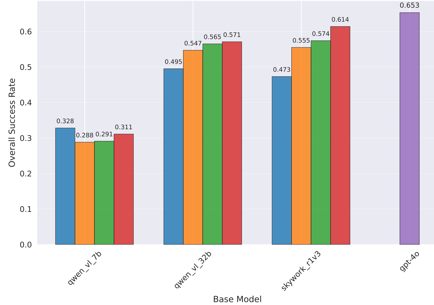
Success Rate Comparison
