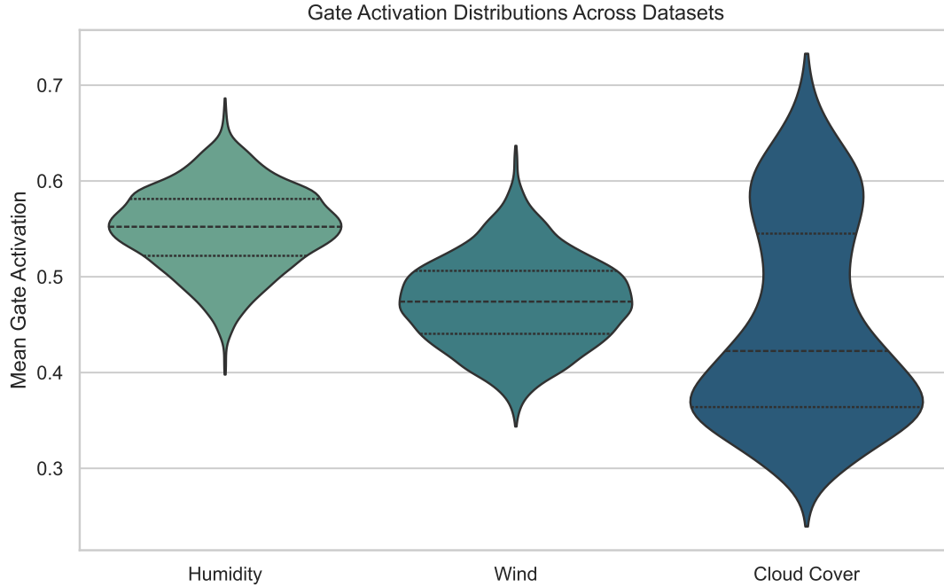
Figure 2. Distribution of mean gate activations for three tasks in a representative trained model. The plot describes how the learned mixture varies across samples. It should not be interpreted as proof that either branch corresponds to a specific physical process.
